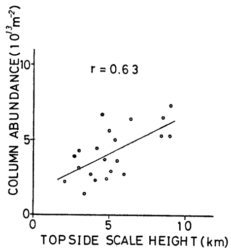
Fig. 6. Correlation between the top side scale height and the column abundance.
