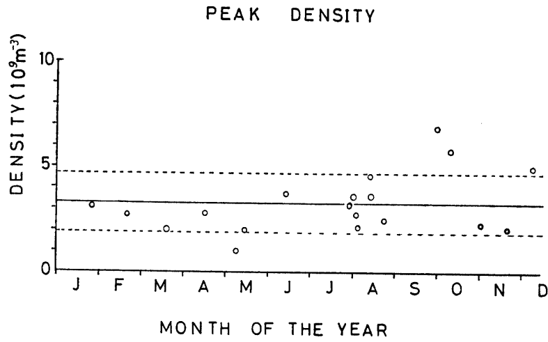
Fig. 3. Seasonal variation of the maximum density of the Na layer. See also the caption of Fig. 2.
