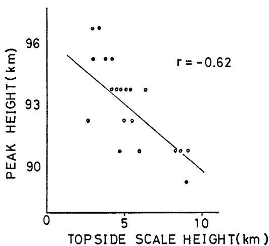
Fig. 7. Correlation between the top side scale height and the peak height.
