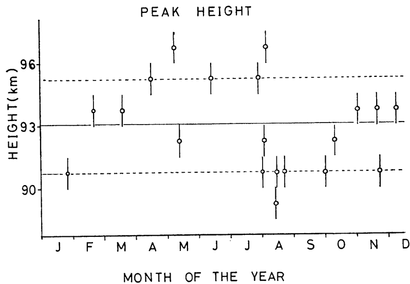
Fig. 2. Seasonal variation of the height of the maximum density. The solid line represents the average and the dashed lines are one standard deviation above and below the average.
