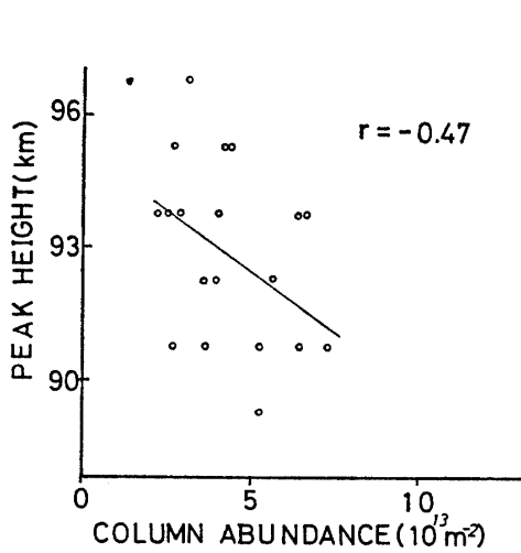
Fig. 5. Correlation between the column abundance and the peak height.
