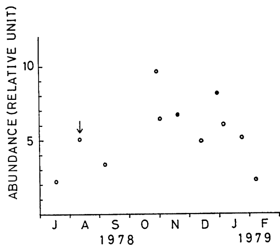
Fig. 8. Seasonal variation of Na total column abundance (relative unit) (1978–79). The open circles indicate good tuning and the closed circles are bad tuning. The arrows correspond to anomalous values correlated with the Perseids meteor shower (after NAGASAWA et al. , private communication, 1979).
