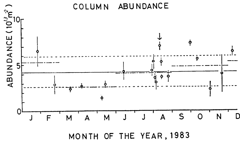
Fig. 1. Seasonal variation of Na total column abundance (1983). The arrows correspond to anomalous values correlated with the Perseids meteor shower. The solid line represents the average, the dashed lines are one standard deviation above and below the average and the dashed-and-dotted lines are the average over three months.
