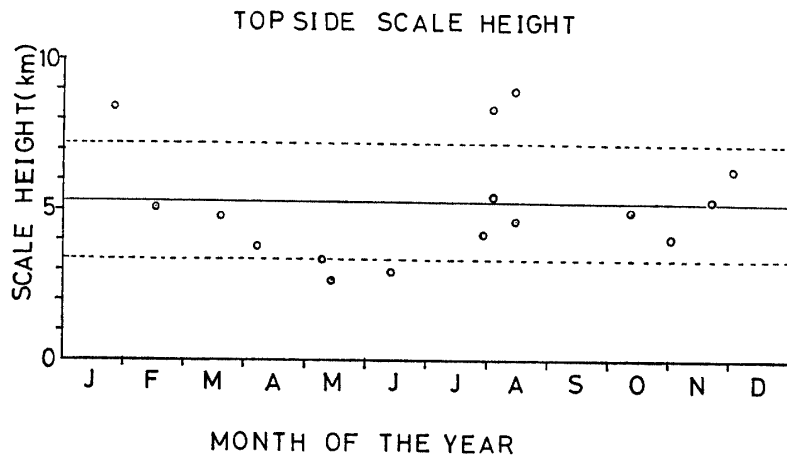
Fig. 4. Seasonal variation of the top side scale height. See also the caption of Fig. 2.
