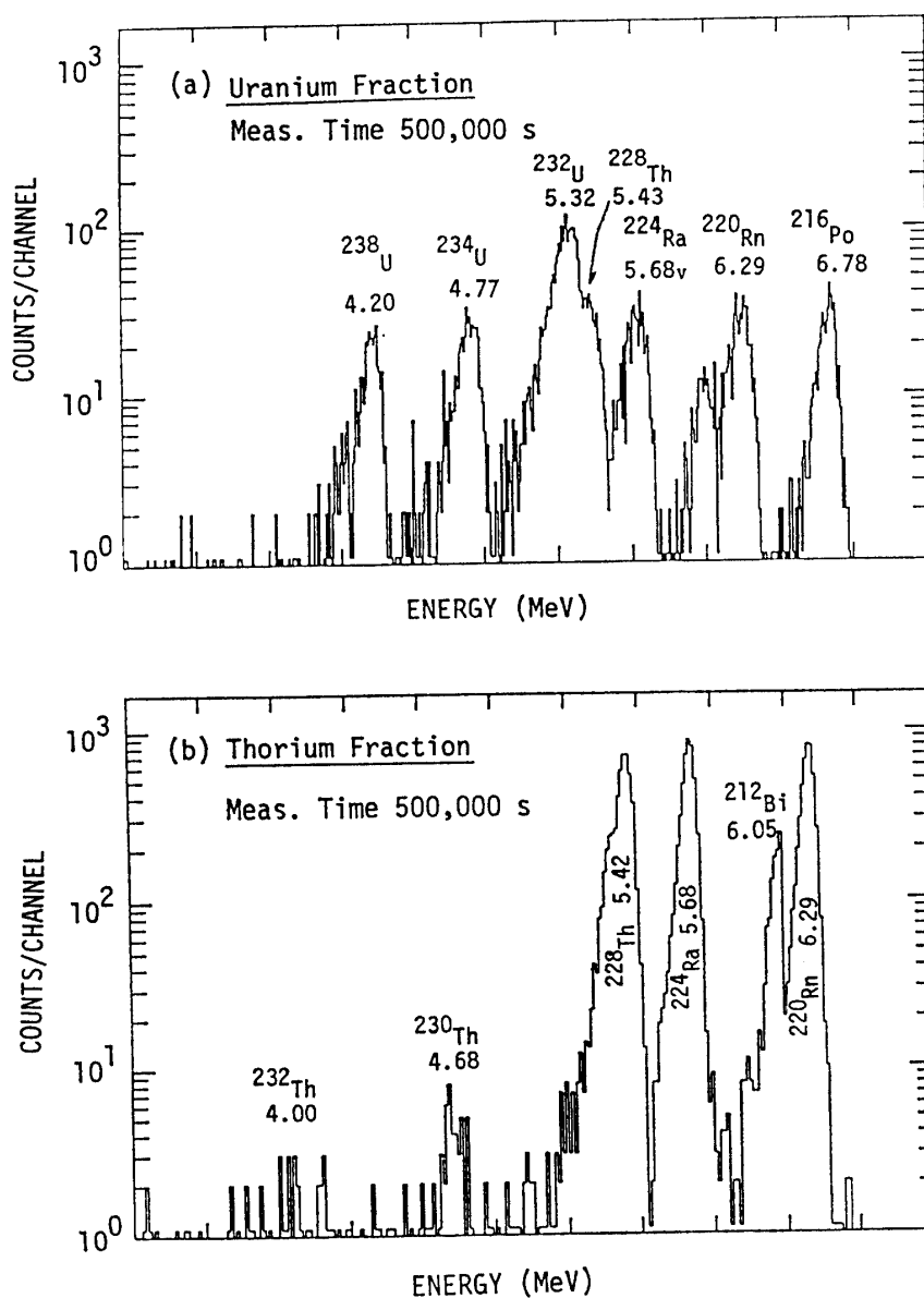
Fig. 2. (a) \alpha -ray spectrum of uranium fraction. (b) \alpha -ray spectrum of thorium fraction.
