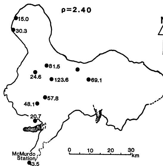
Fig. 5. Bouguer anomaly in Ross Island. Basement density \rho = 2.40 \text{ Mg/m}^3 .
