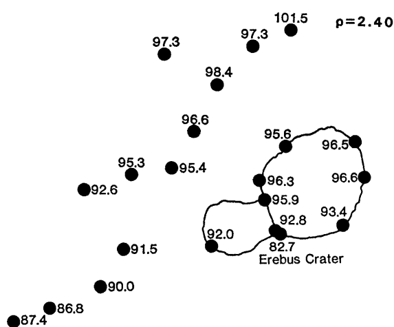
Fig. 2. Bouguer anomaly in the summit area. Basement density \rho=2.40 \text{ Mg/m}^3 .
