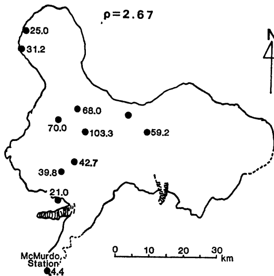
Fig. 4. Bouguer anomaly in Ross Island. Basement density \rho = 2.67 \text{ Mg/m}^3 .
