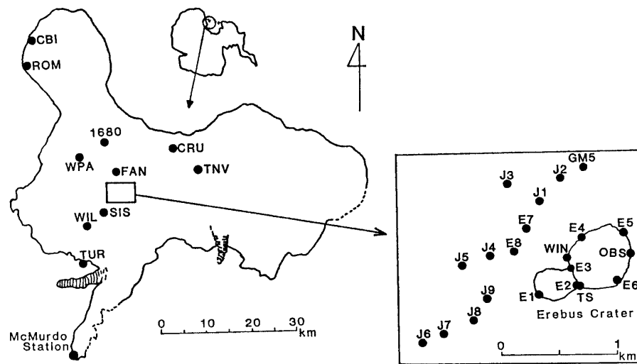
Fig. 1. Locations of gravity stations in Ross Island, Antarctica.
