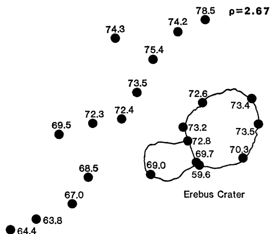
Fig. 3. Bouguer anomaly in the summit area. Basement density \rho=2.67 \text{ Mg/m}^3 .
