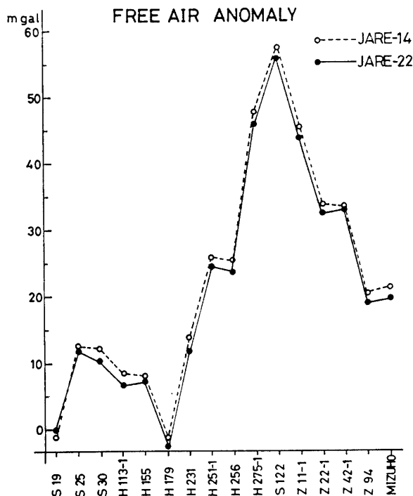
Fig. 5. Free air anomalies between Syowa and Mizuho Stations along the snow traverse route by JARE-14 and -22.
