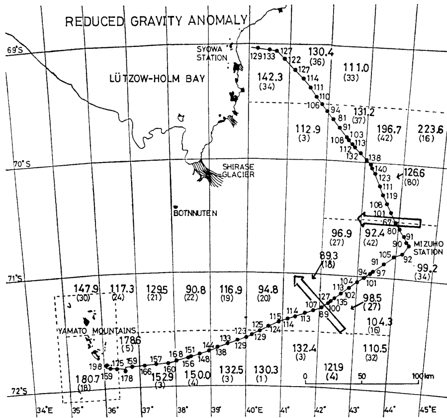
Fig. 2. The reduced gravity anomaly in the Mizuho Plateau. The values indicated by larger letters and the number in parentheses are the averaged reduced gravity anomalies and the number of stations in the area of 1° in longitude and 0.5° in latitude by KAMINUMA (1979). Large open arrows are the locations of estimated subglacial valleys and their flow directions.
