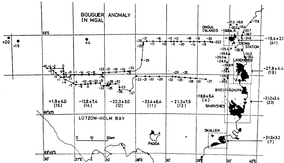
Fig. 1. Simple Bouguer anomalies on the sea ice and in the ice-free areas of Lützow-Holm Bay. The three data indicated by large solid circles were obtained by OURA (1965). The areas enclosed by dotted lines show the ice-free areas. The values indicated by small solid circles on solid lines are the data on the sea ice. Solid triangles and solid circles are the measurement at triangulation points on islands and other small exposed areas, respectively.
