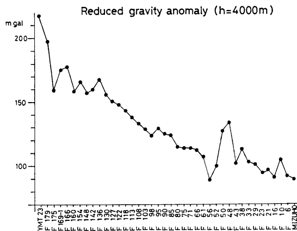
Fig. 3. The reduced gravity anomaly between Mizuho Station and the Yamato Mountains. The points on the abscissa show the station name of over-snow traverse by JARE-22.
