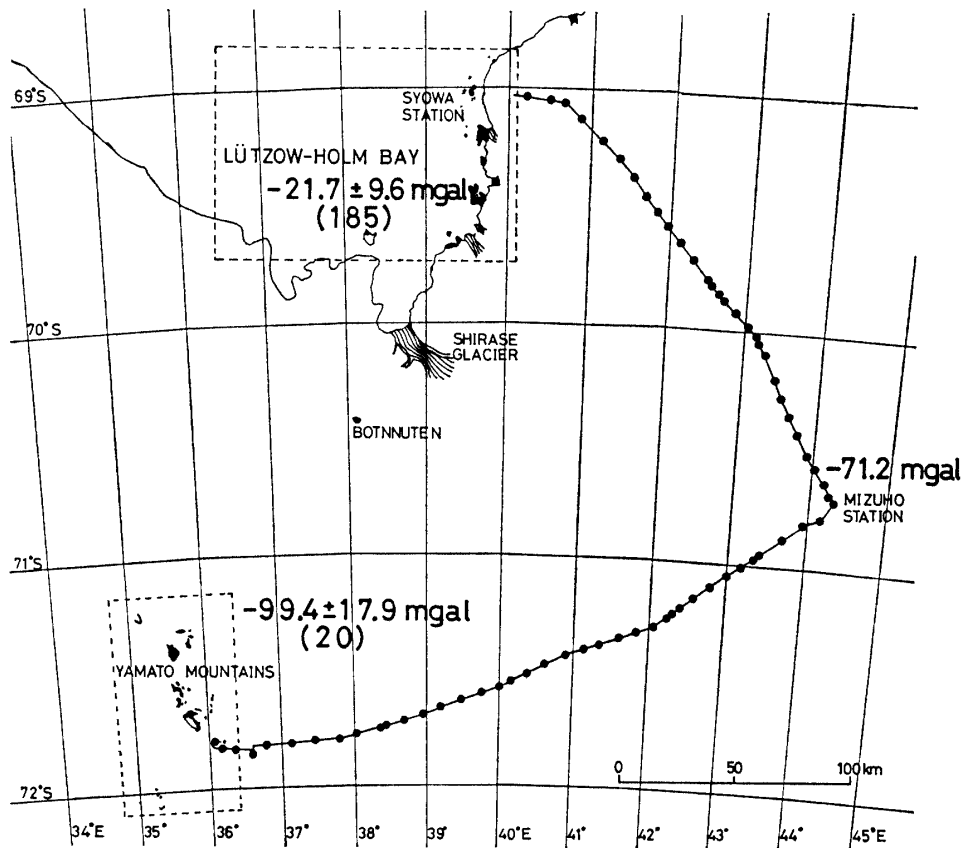
Fig. 4. Averaged simple Bouguer anomalies in the Lützow-Holm Bay region and the Yamato Mountains region, and simple Bouguer anomaly at Mizuho Station. The number in parentheses is the number of stations in each enclosed area by dotted line.
