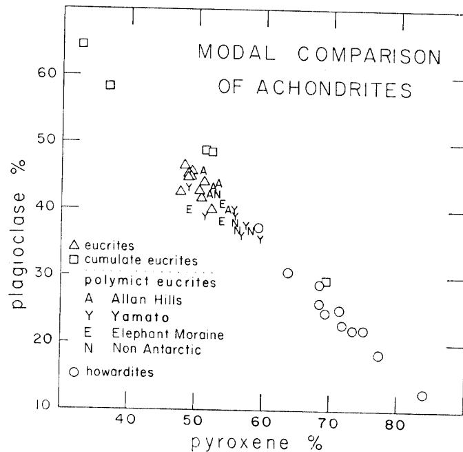
Fig. 1. Modal plagioclase vs. total pyroxene content of Yamato and Allan Hills polymict eucrite specimens compared with howardites, eucrites and cumulate eucrites. Data for Elephant Moraine and non-Antarctic polymict eucrites are also shown.
