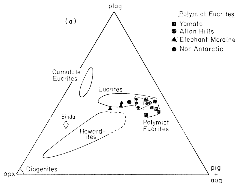
Fig. 2a. Modal orthopyroxene—“clinopyroxene”—plagioclase ternary diagram for Yamato and Allan Hills polymict eucrites compared with other basaltic achondrites. In this figure all modal “pigeonite” is assumed to be true pigeonite clinopyroxene.
