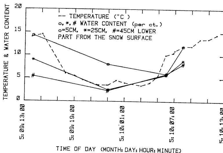
Fig. 3. Diurnal variations of the air temperature and the water content.
