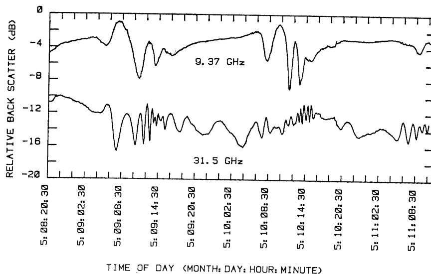
Fig. 2. Diurnal variations of the relative intensity of the back scatter.
