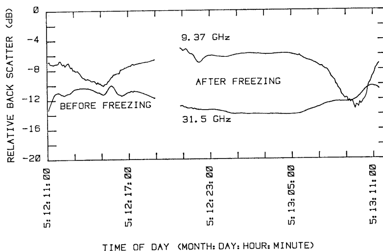
Fig. 4. Variations of the back scatter from wet and frozen snowpack.
