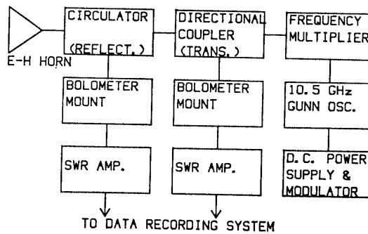
(B) R-BAND WAVEGUIDE SYSTEM
