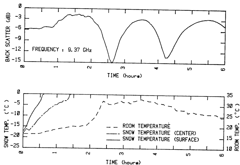
Fig. 5. Variations of the intensity of back scatter of 9.37 GHz wave and the room and snow temperatures against the time.
