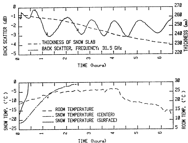
Fig. 7. Relations between the thickness of snow slab and the periodic fluctuation of the back scatter at the frequency of 31.5 GHz.
