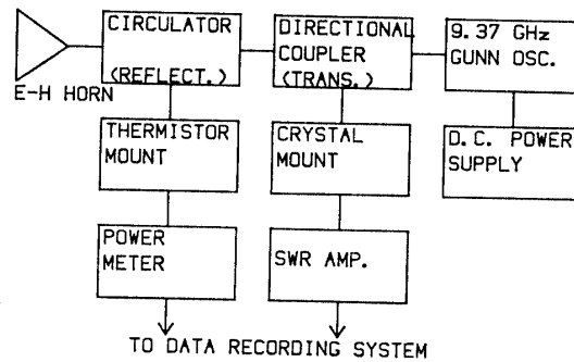
(A) X-BAND WAVEGUIDE SYSTEM
