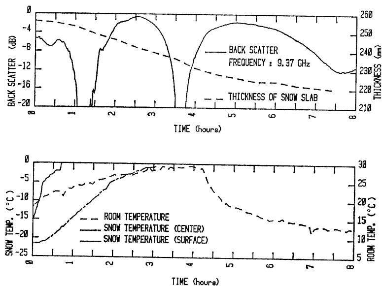
Fig. 8. Relations between the thickness of snow slab and the periodic fluctuation of the back scatter at the frequency of 9.37 GHz.
