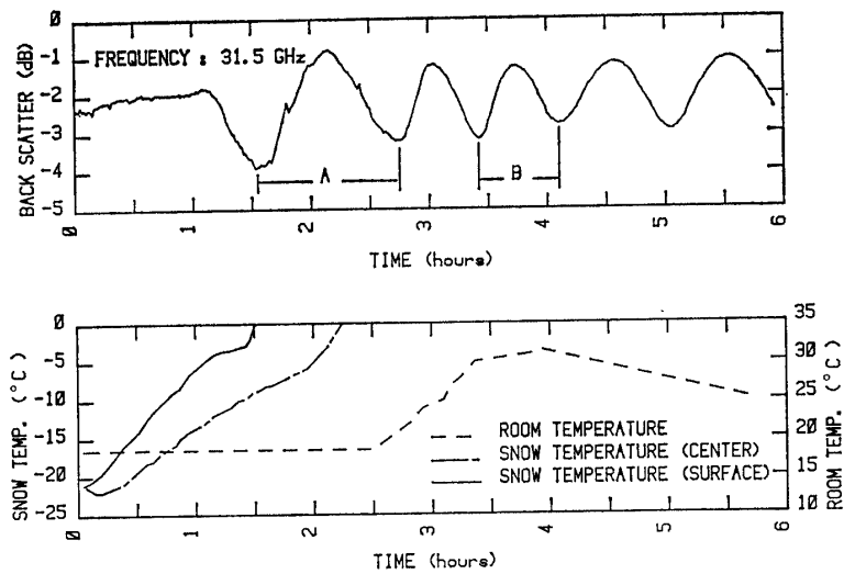
Fig. 6. Variations of the intensity of back scatter of 31.5 GHz wave and the room and snow temperatures against the time.
