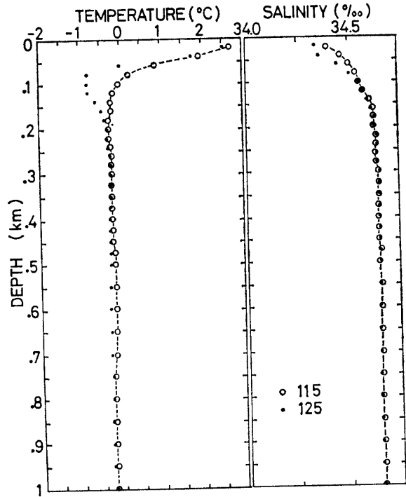
Fig. 7. A comparison of profiles of vertical temperature and salinity at station 115 (open circles) and station 125 (dots) of the ISLAS ORCADAS.
