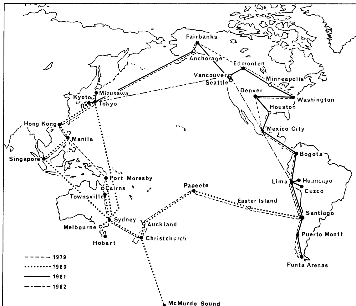
Fig. 1. Routes and cities occupied by the international gravimetric connections around the Circum-Pacific zone.
