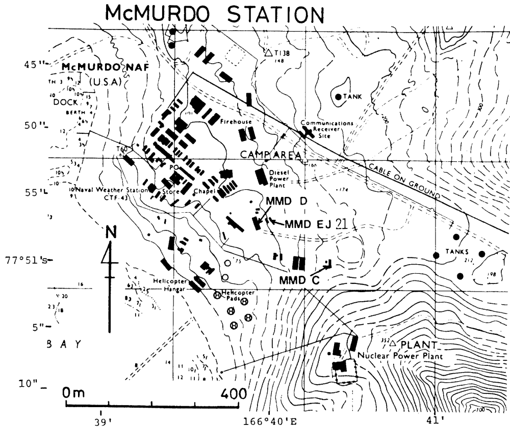
Fig. 2a. Location map of measuring stations in McMurdo Station.
