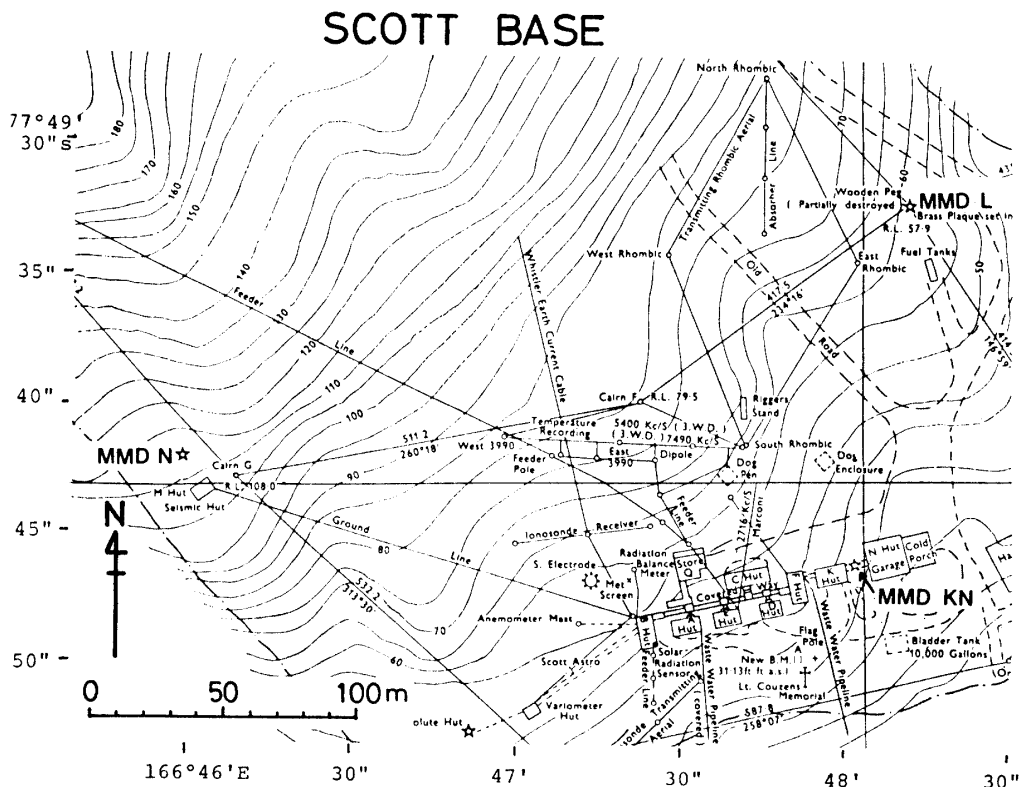
Fig. 2b. Location map of measuring stations in Scott Base.
