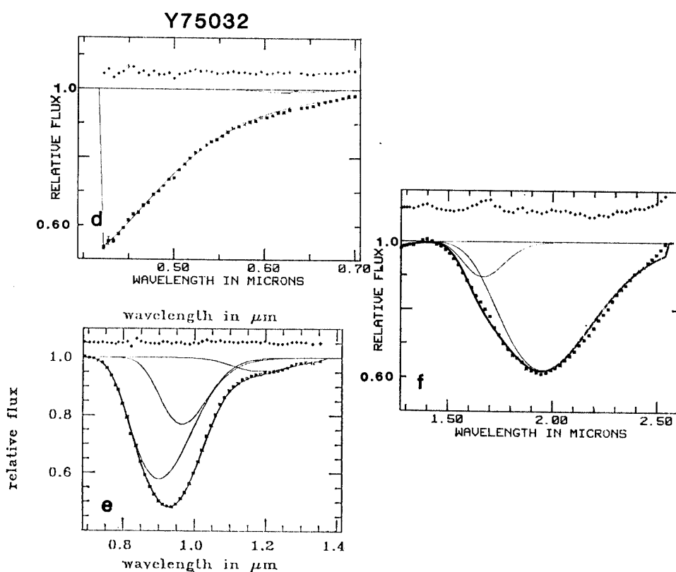
Fig. 2. d) same as (a) for Y-75032 visible spectrum. The 0.50- \mu\text{m} band cannot be fit but can be detected as a negative residual. e) Two pyroxene bands and 1 plagioclase band are resolved in the 0.9- \mu\text{m} region spectrum of Y-75032. f) The 2.0- \mu\text{m} region of Y-75032.
