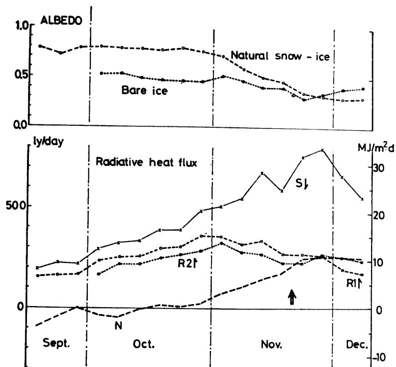
Fig. 2. Mean values of radiation components for every 5 days at sites (A) and (B) in 1980.
