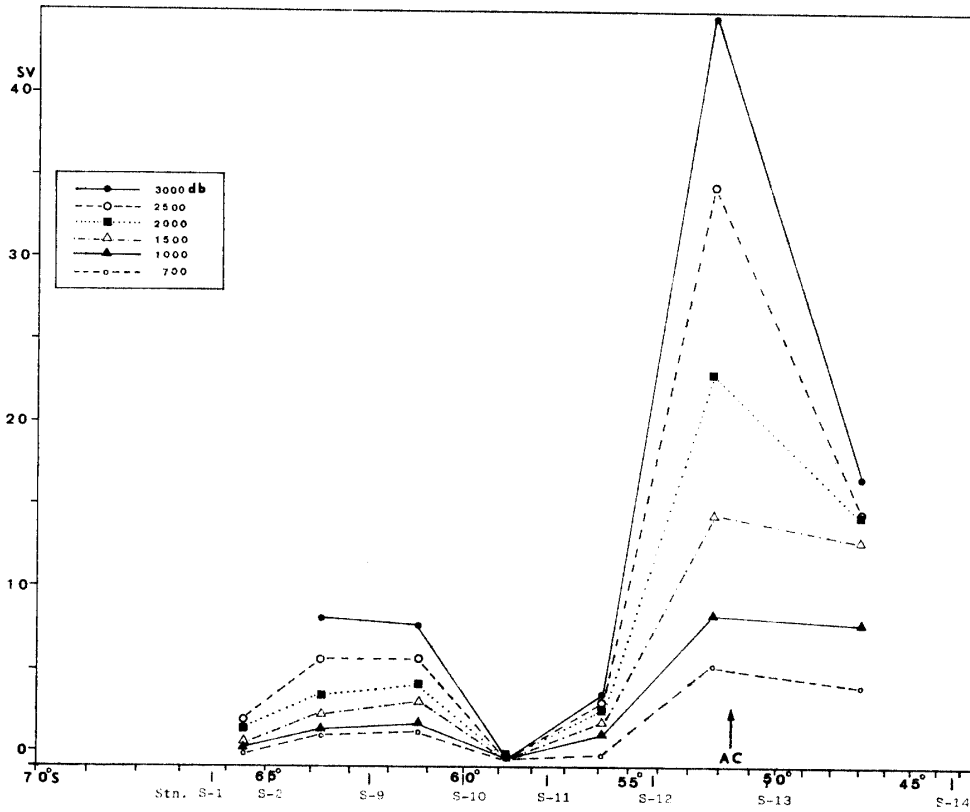
Fig. 4. Geostrophic volume transport at 45°E for the selected reference level.
