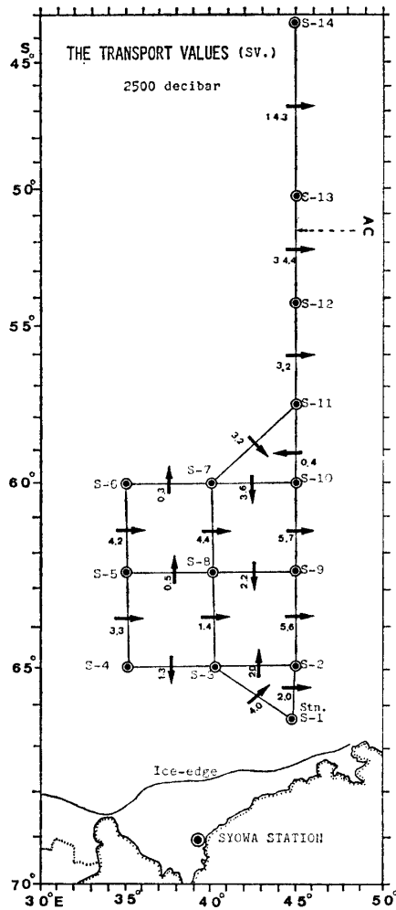
Fig. 3. Geostrophic volume transport referred to 2500 db surface in sv ( 1 \text{ sv} = 10^6 \text{ m}^3/\text{s} ).
