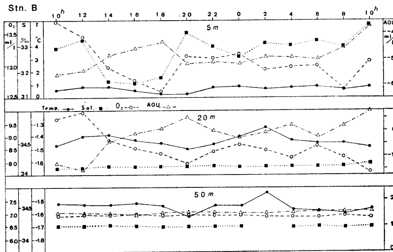
Fig. 7. Time variation of temperature, salinity, dissolved oxygen content and AOU for three layers at Stn. B.
