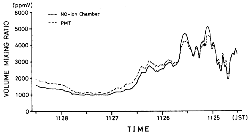
Fig. 7. The results of conversion of the data shown in Fig. 6 into the volume mixing ratio of water vapor. The accurate data reduction method described in the Section 2 was applied to obtain the results shown by the broken line. The results shown by the solid line were deduced from the absolute humidity obtained with the NO-ion chamber using the air density values of the US Standard Atmosphere, 1976.
