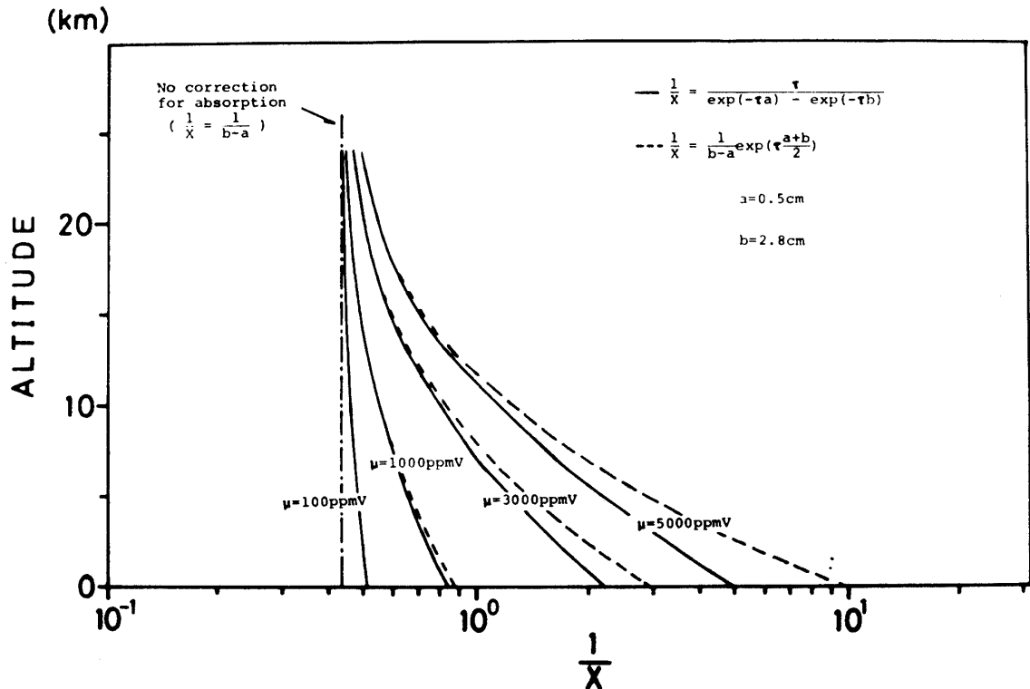
Fig. 3. The values of 1/X in eq. (4) versus altitude for various volume mixing ratios of water vapor. The number density of air molecules is based upon the model atmosphere (US Standard Atmosphere, 1976).
