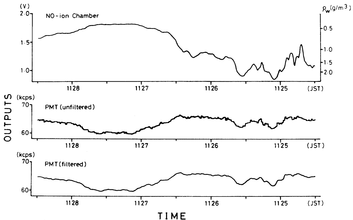
Fig. 6. Typical output of the instrument for the aircraft observations (June 24, 1981, over Mikawa district). The upper panel shows logarithmically amplified output of the NO-ion chamber. Right ordinate indicates absolute humidity. The middle panel shows direct output of the photon counter. The left ordinate indicates counting rates. The lower panel shows outputs of the photon counter smoothed by a lowpass filter whose cut-off frequency is 0.2 Hz.
