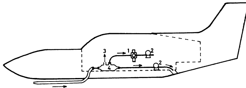
Fig. 5. Schematic representation of the method of air sampling in the aircraft observation. 1. Sensing unit of the instrument, 2. Pump, 3. Air sample opening for other research, 4. Air sample chamber, → Air flow.
