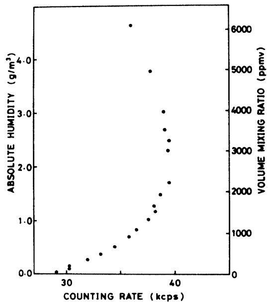
Fig. 2. Output counting rate of the photon counter versus water vapor in the air (IWASAKA et al., 1981). Calibration curves can be varied by using various arrangements of individual components in the sensing unit.
