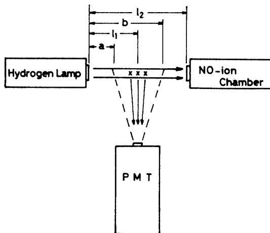
Fig. 1. Schema of the principle of the instrument.
