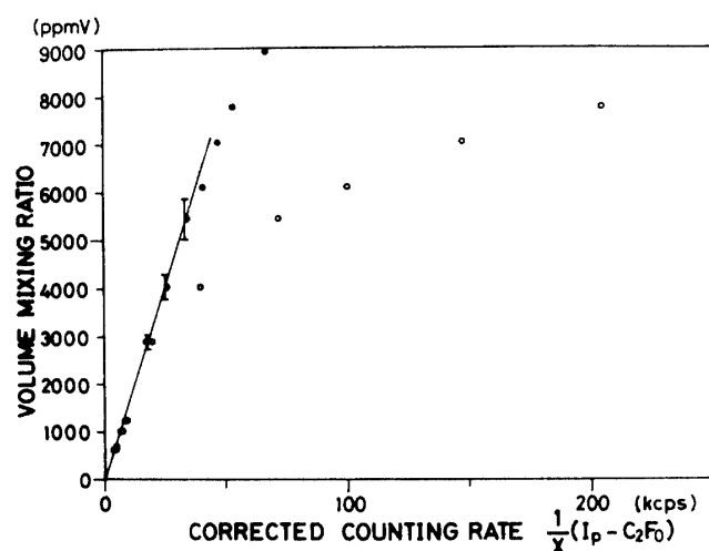
Fig. 4. Corrected counting rate versus the volume mixing ratio of water vapor. The filled circles give the correction based upon eq. (3b), and the open circles the correction based upon eq. (5a). The I on the fitting line indicates the error range corresponding to an error of \pm 0.5 kcps in the value of original counting rate I_p .
