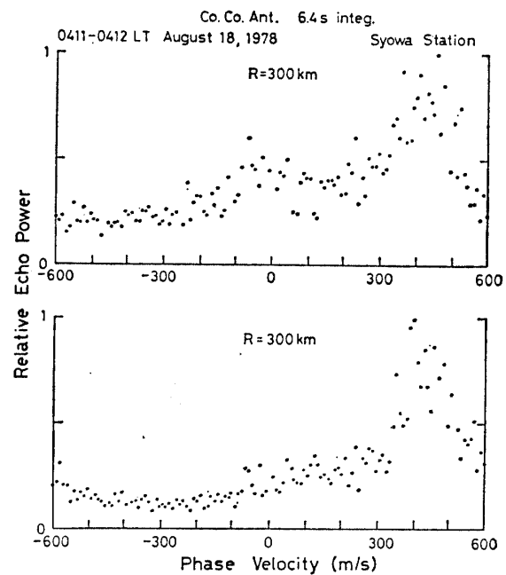
Fig. 6. Echo power spectra obtained during 0411–0412 LT on August 18, 1978. Power spectra were taken at 300 km range with PRF=330 Hz and coaxial collinear receiving antenna. The dominant doppler shift is seen approximately at 450 m/s corresponding to the electric field component of about 23 mV/m. The upper figure precedes the lower figure in time.
