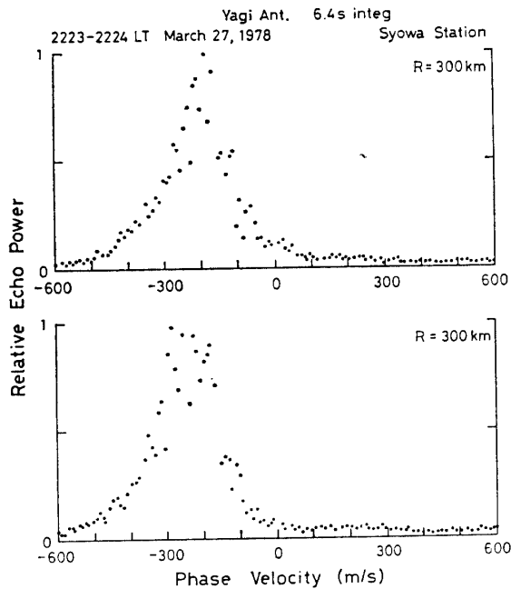
Fig. 9. Echo power spectra obtained during 2223–2224 LT on March 27, 1978. Power spectra were taken at 300 km range with PRF=400 Hz and Yagi receiving antenna. The dominant doppler shift is seen approximately at -250 m/s corresponding to the electric field component of about 13 mV/m. The upper figure precedes the lower figure in time.
