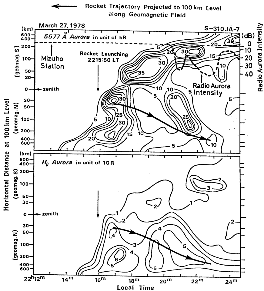
Fig. 8. Contours of 5577 \text{ \AA} aurora and H_{\beta} aurora measured by scanning photometer at Syowa Station. The S-310JA-7 rocket trajectory projected down to 100 km level along the geomagnetic field is also shown. Time variation of auroral radar echo intensity over Mizuho Station is represented by a thick broken curve.
