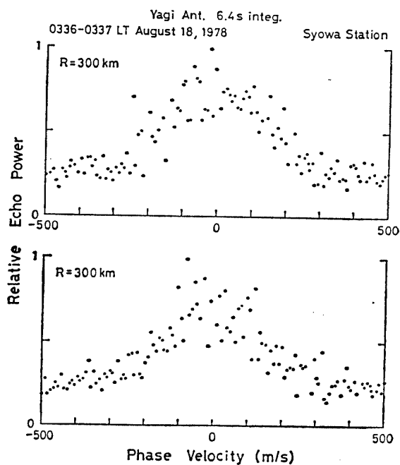
Fig. 4. Echo power spectra obtained during 0336-0337 LT on August 18, 1978. Power spectra were taken at 300 km range with PRF=330 Hz and Yagi receiving antenna. The upper figure precedes the lower figure in time.
