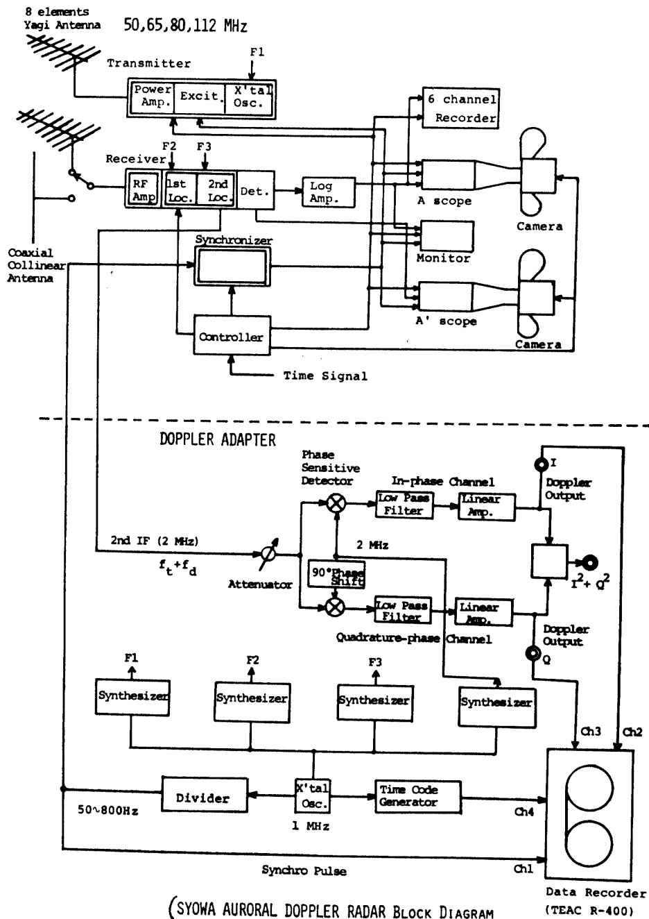
Fig. 1. System block diagram of the auroral doppler radar. Yagi antenna is used for the transmitting antenna. Yagi antenna is usually used for the receiving antenna, and a coaxial collinear antenna is occasionally used for the receiving antenna. Signal scattered from ionospheric irregularities is recorded on the analog data recorder.
