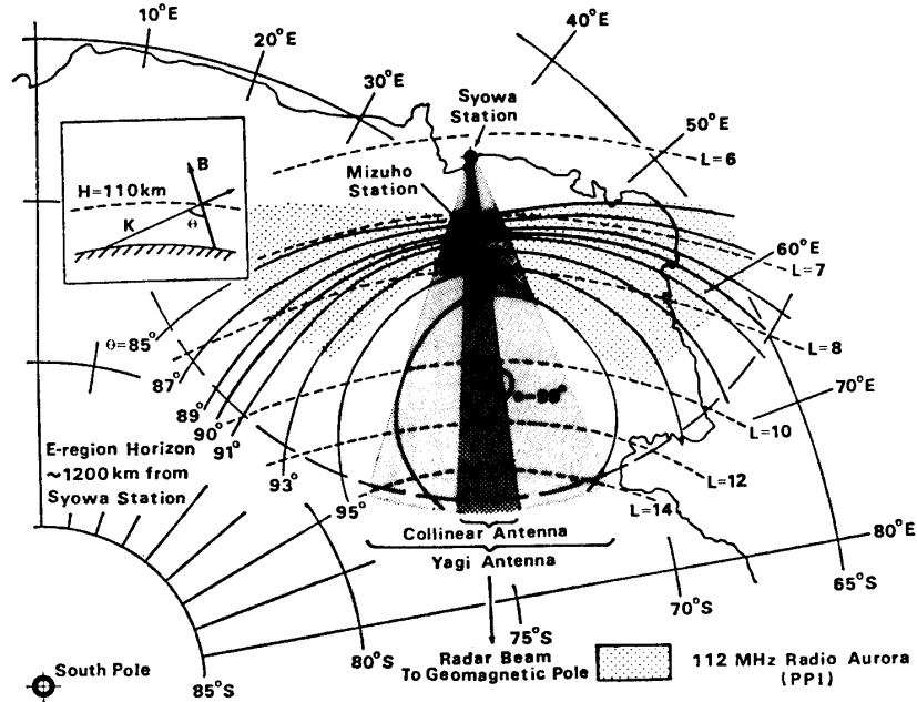
Fig. 2. Plan view of radar antenna patterns (Yagi and collinear antennas) together with contours of L value and aspect angle \theta . The aspect contours are shown for a height of 110 km. The dotted-area represents the echo region of 112 MHz radio aurora.
