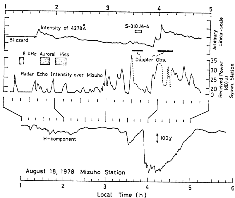
Fig. 3. Time profiles of 50 MHz radar echo intensity received at Syowa Station, optical aurora intensity ( 4278 \text{ \AA} ) observed by the photometer and geomagnetic H -component at Mizuho Station. The doppler radar was operated during the time interval indicated by a thick line. The S-310JA-4 rocket was launched at 0332:43 LT on August 18, 1978.
