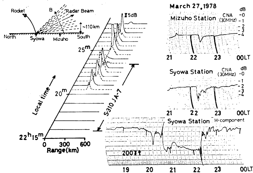
Fig. 7. Time variation of A-scope display of the 50 MHz radio aurora when S-310JA-7 was launched at 2215:50 LT on March 27, 1978. Geomagnetic H-component at Syowa Station, and 30 MHz cosmic noise absorption at Mizuho and Syowa Stations are shown on the right.
