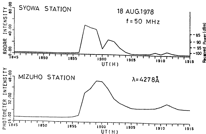
Fig. 5. Radio aurora intensity (50 MHz) and optical aurora intensity (4278 Å) measured when the auroral arcs passed over Mizuho Station. The time resolution of the record is one minute.
