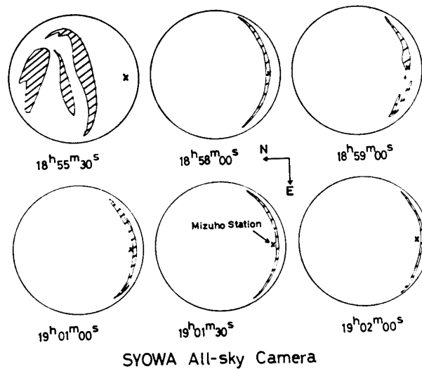
Fig. 7. Schematic all-sky photographs at Syowa Station from 1855:30 to 1902:00 UT on August 18, 1978. The hatched-area shows the region of visible aurora.
