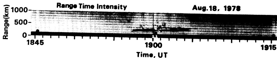
Fig. 6. Range-time-intensity of the radio aurora from 1845 to 1915 UT on August 18, 1978. The black stripes show the echo region.
