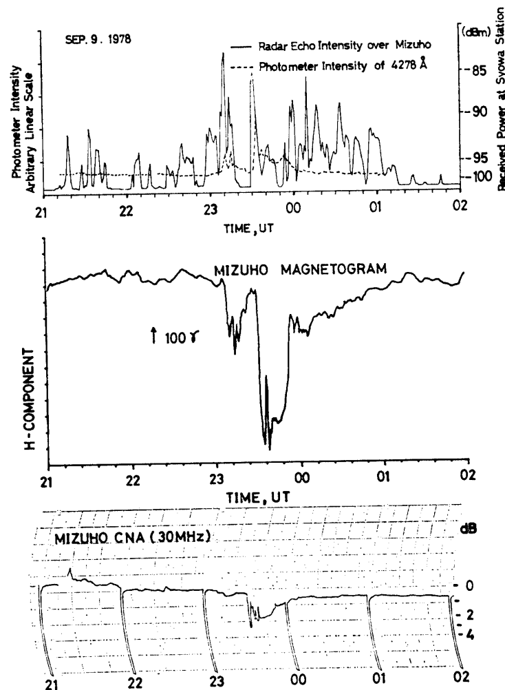
Fig. 4. Radio aurora intensity (50 MHz) and optical aurora intensity (4278 Å) [top], magnetic H-component at Mizuho Station [middle], and 30 MHz riometer record at Mizuho Station [bottom] on September 9, 1978.
