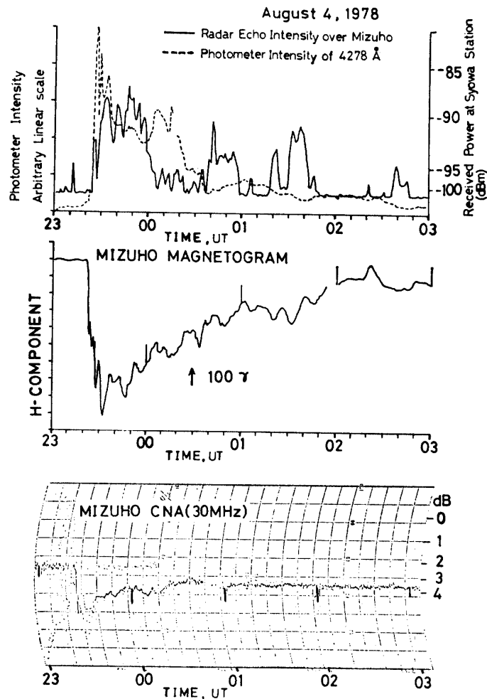
Fig. 3. Radio aurora intensity (50 MHz) and optical aurora intensity (4278 Å) [top], magnetic H-component at Mizuho Station [middle], and 30 MHz riometer record at Mizuho Station [bottom] on August 4, 1978.
