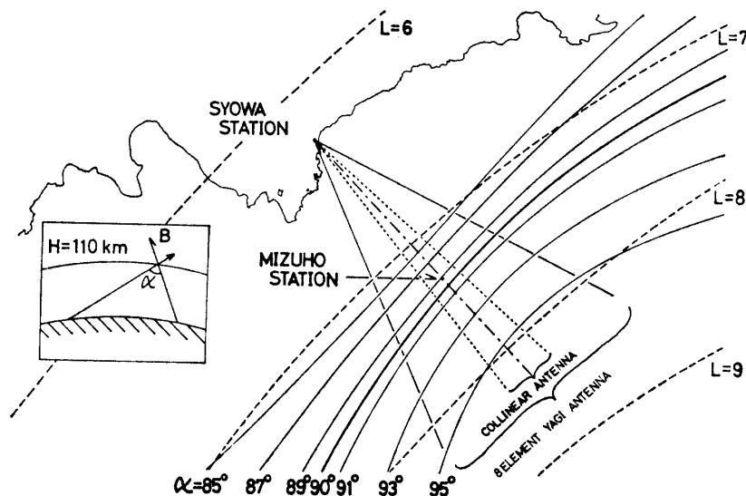
Fig. 1. Plan view of auroral radar antenna patterns along with contours of L value and aspect-angle for a height of 110 km. The inset defines the aspect angle \alpha .
