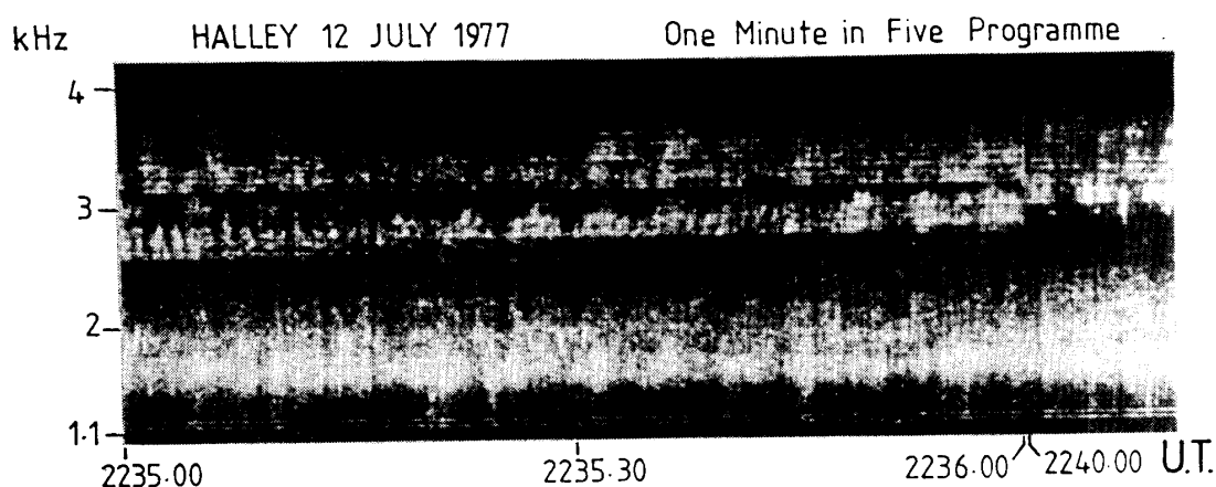
Fig. 7. Data recorded on a one minute in five sampling program, showing how line arrays can develop over the time period of minutes. Between 2235.00 and 2236.00 the line radiation is split into two distinct bands (centred on \sim 2.8 and 3.2 kHz), whereas at the start of the 2240-41 run these bands have apparently merged together.
