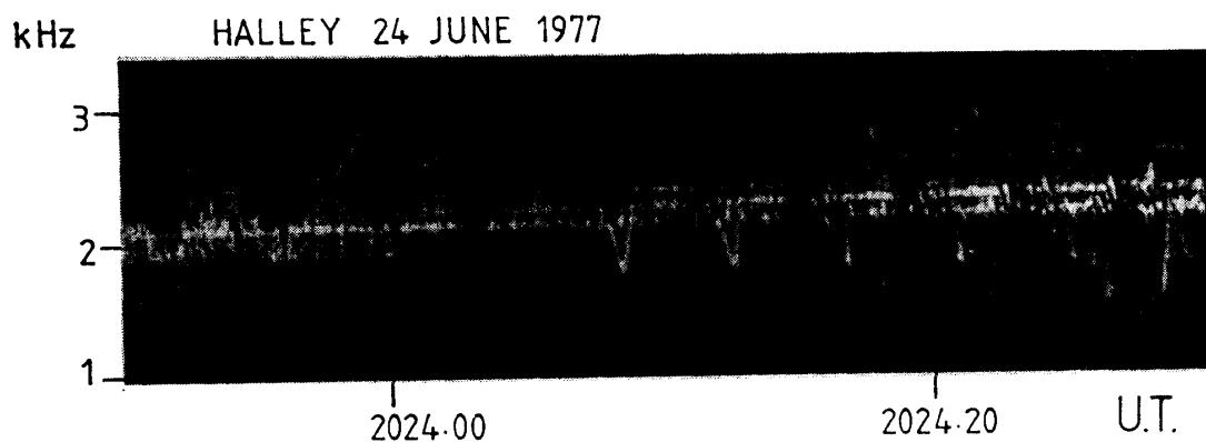
Fig. 4. The three magnetospheric lines illustrated here all drift at different rates. The lower line triggers several well defined hooks, and a clear two hop amplitude modulation is visible.
