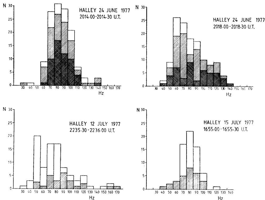
Fig. 8. Histograms showing the distribution in frequency of separation between adjacent magnetospheric lines. Key:—
