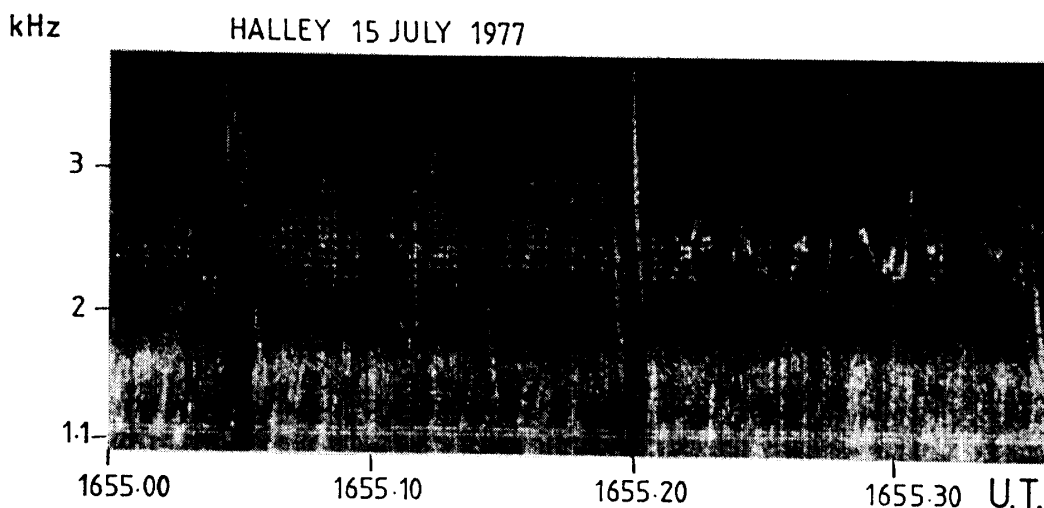
Fig. 5. Magnetospheric line array centred on \sim 2.5 kHz. Two hop amplitude modulation is visible. At 1655.05 UT and 1655.20 UT two very loud whistlers overload the receiving apparatus and cause a data drop out at lower frequencies. After 1655.22 UT the line radiation event dies out and emissions are triggered from the frequencies previously occupied by the lines.
