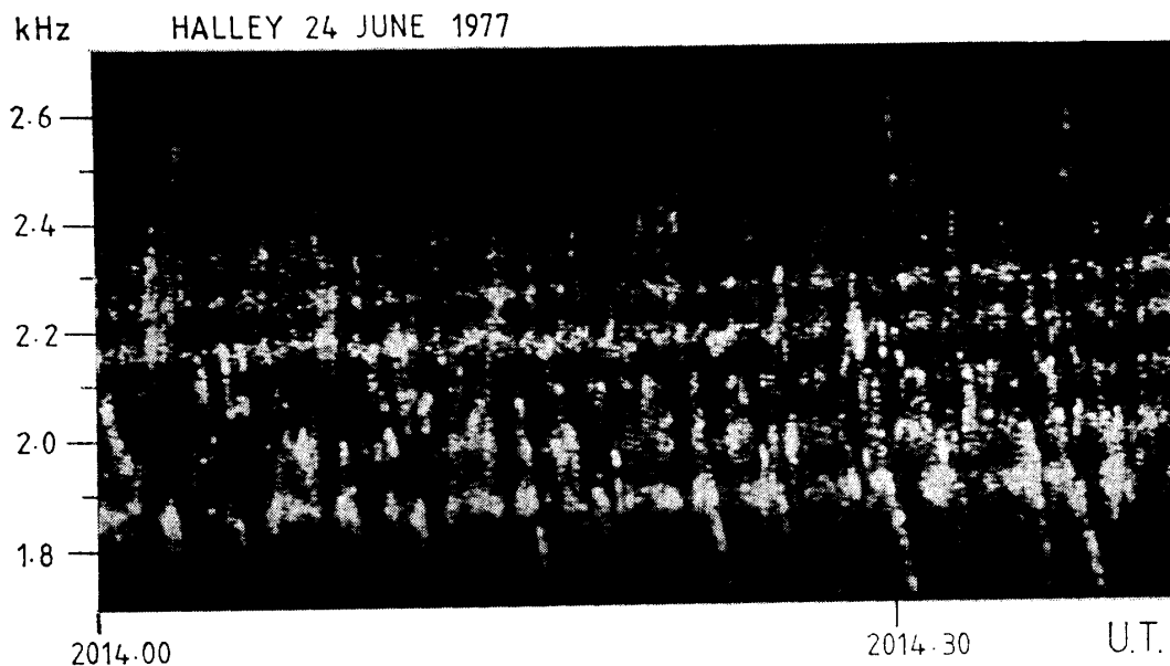
Fig. 3. Spectrogram on an expanded frequency scale showing magnetospheric lines in greater detail (resolution \sim 2 Hz). Line frequency drifts, small scale amplitude fluctuations, and triggering of risers and fallers are exhibited.
