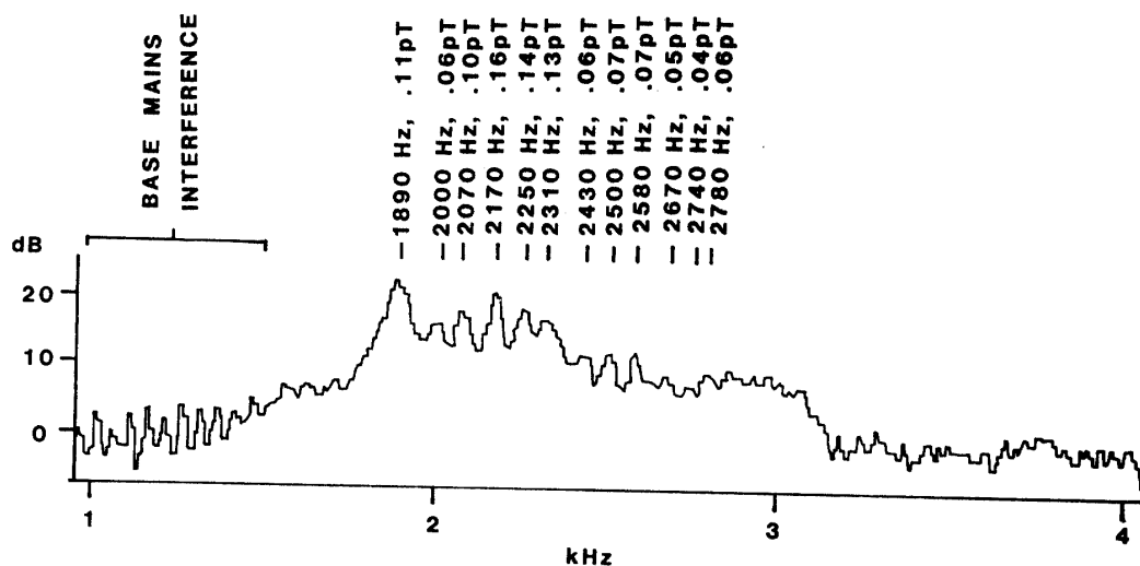
Fig. 2. Amplitude (log. scale) versus frequency plot of the 3 second portion of data between 2014.08 and 2014.11 UT on 24 June 1977 (see Fig. 1). Interference from the local power system at Halley appears as a series of well defined spikes near 1.2 kHz. The magnetospheric lines starting at 1.89 kHz are of broader bandwidth ( \sim 30 Hz), and greater signal intensity (.16 pT max).
