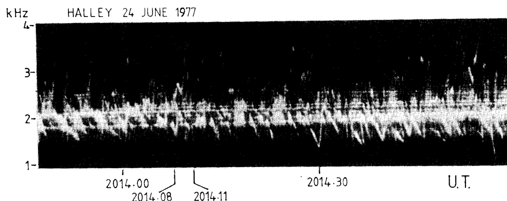
Fig. 1. The spectrogram shows a well defined array of magnetospheric lines which are gradually drifting up in frequency at \sim 80 Hz/min, and lie in the frequency range 1.75–2.5 kHz. The lines trigger emission activity and show some evidence of a two hop modulation in the envelop of the wave spectrum. Local induction lines from Halley station are just visible between 1–1.5 kHz, and are regularly spaced lines of constant frequency.
