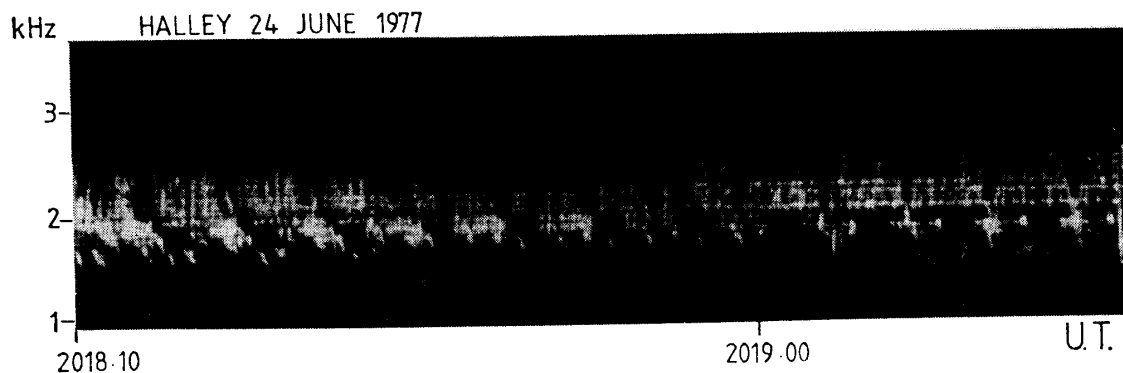
Fig. 6. Well defined and intense band of line radiation exhibiting extensive triggering of emissions.
