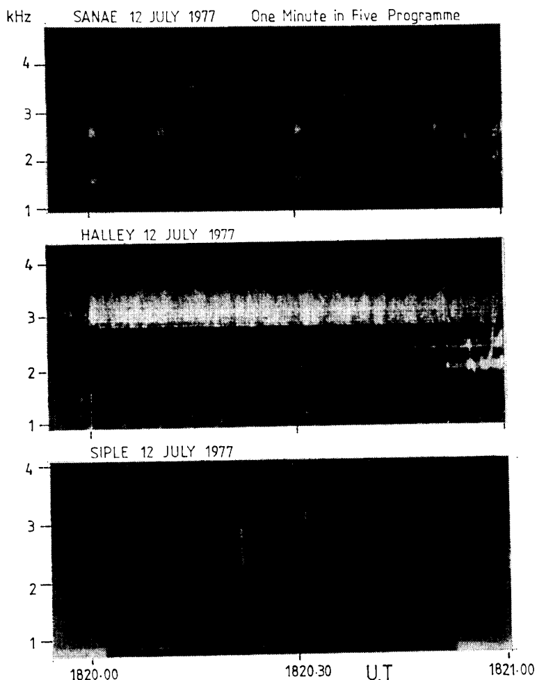
Fig. 9. Spectrograms from Halley ( L=4.3 ), Sanae ( L=4.1 ) and Siple ( L=4.0 ). On the Halley record an intense hiss band is visible at around 3 kHz. Line structure is present in this band. Two whistlers are recorded at \sim 1820.22 and \sim 1820.31 UT. On the Sanae record the line structured hiss band is visible, though less intense than at Halley, but the two whistlers are not visible. The Siple data show these two whistlers quite clearly but the structured hiss band is barely visible.
