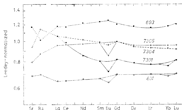
Fig. 2. The Leedey-normalized REE patterns of five Antarctic chondrites analyzed by MASUDA et al. (1977) and by MASUDA and TANAKA (1978).
