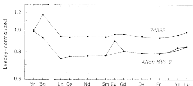
Fig. 1. The Leedey-normalized REE patterns for two chondrites studied in the present study; the normalizing value, 11.1 ppm, for Sr is from GOPALAN and WETHERILL (1971).
