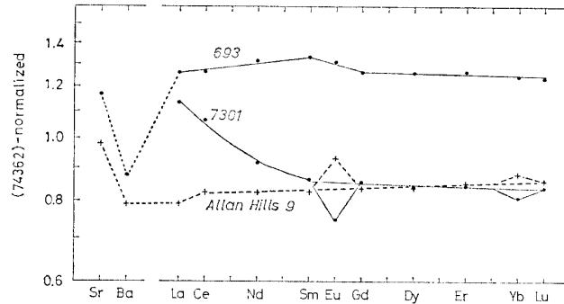
Fig. 3. The REE patterns of chondrites, Yamato-693, -7301 and AH9, normalized by Yamato-74362 in place of the Leedey chondrite.
