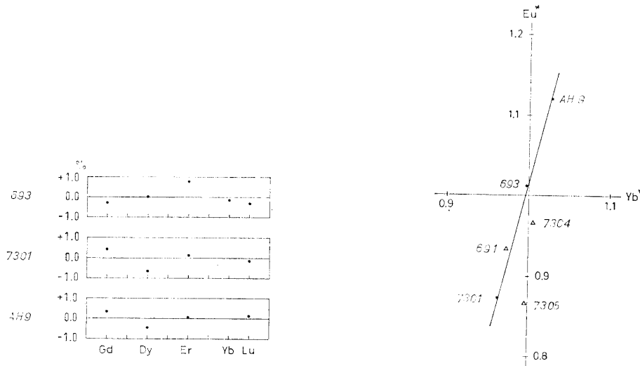
Fig. 4. Demonstration of extent of linearity for heavy REE span on an expanded scale, for each of REE patterns shown in Fig. 3.
