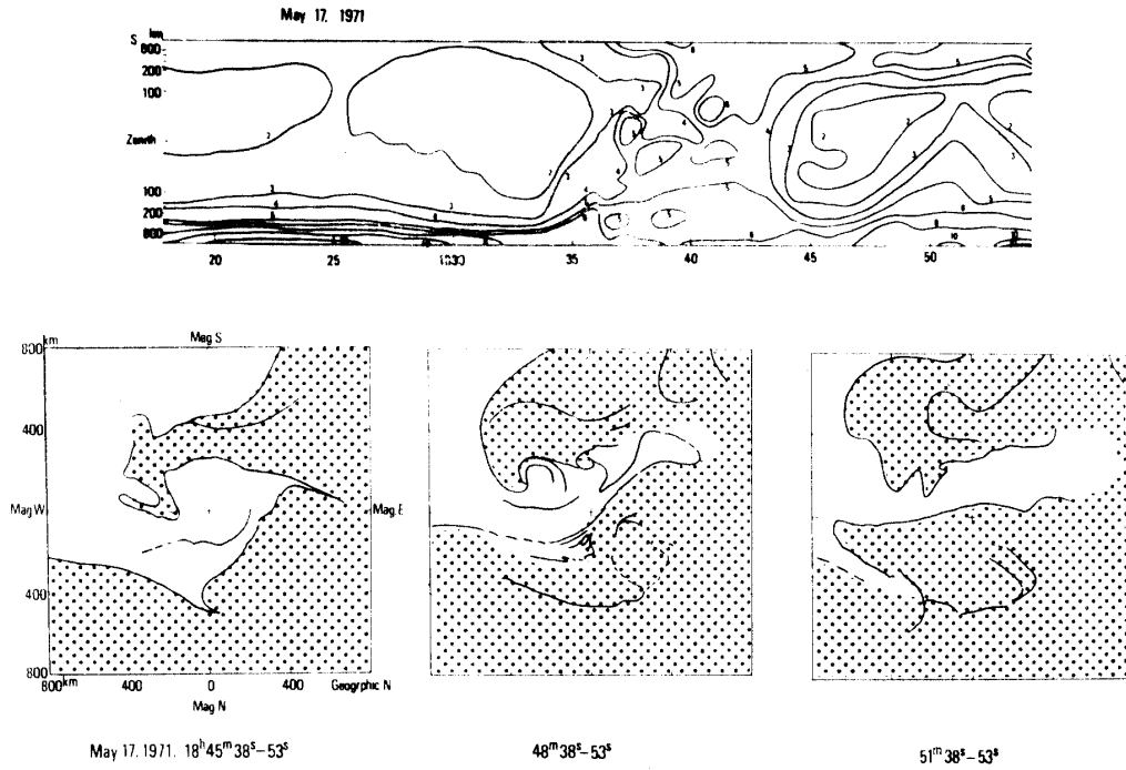
Fig. 3. Development of electron aurora and hydrogen emission during the auroral breakup of May 17, 1971. The figure shows the part of the westward travelling surge of a global auroral activity. Dotted area schematically indicates the region of strong hydrogen emission.
