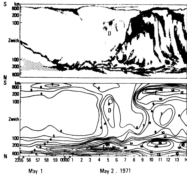
(2b) Top: Meridian-time display of the electron aurora. Bottom: Meridian-time display of hydrogen emission.
