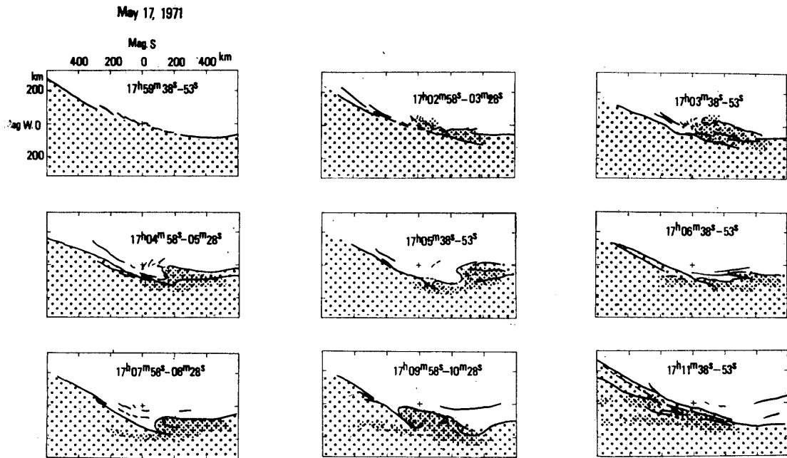
Fig. 5. Development of electron aurora and hydrogen emission during a local breakup which occurred in the evening of May 17, 1971. Though the pattern of the activity is much smaller than the previous examples, the general feature of development closely resembles the latter.
