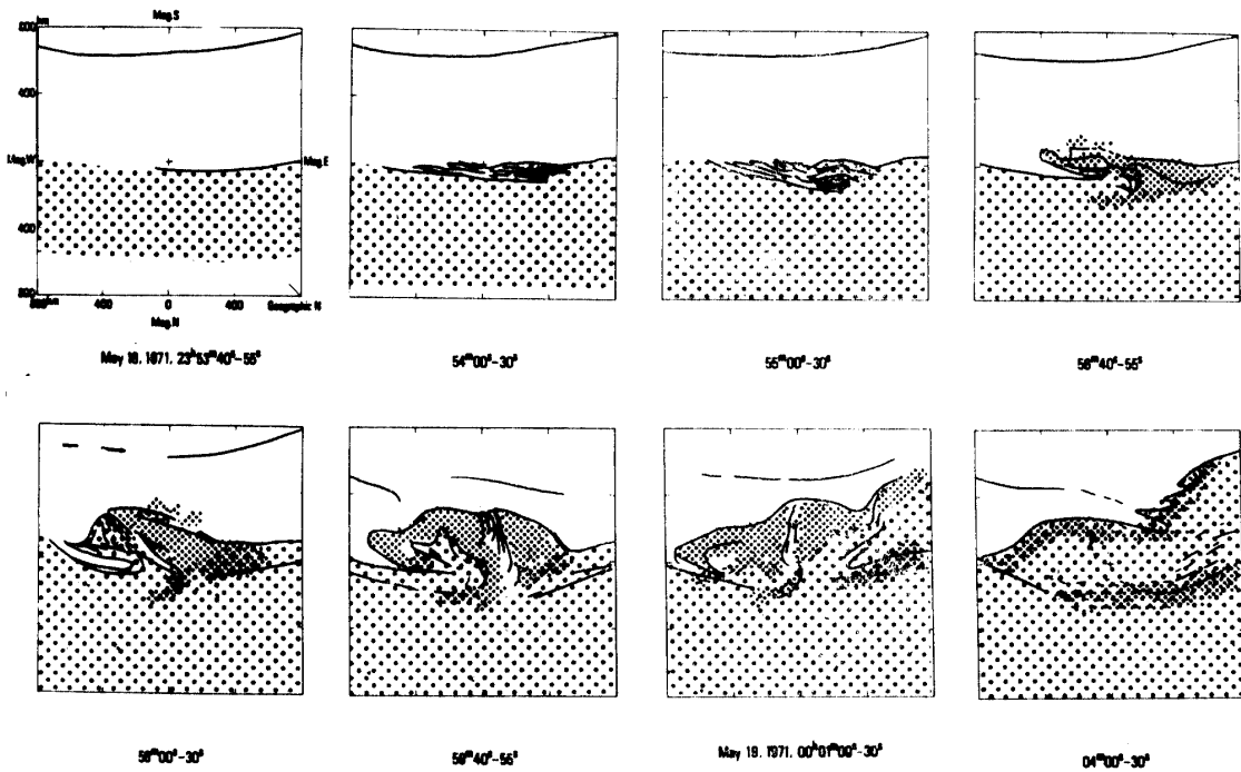
(1c) Linear scale representation of the pattern and development of electron aurora and hydrogen emissions. Dense and sparse dots indicate the regions of strong and weak hydrogen emission, respectively, during the auroral breakup of May 18-19, 1971.
