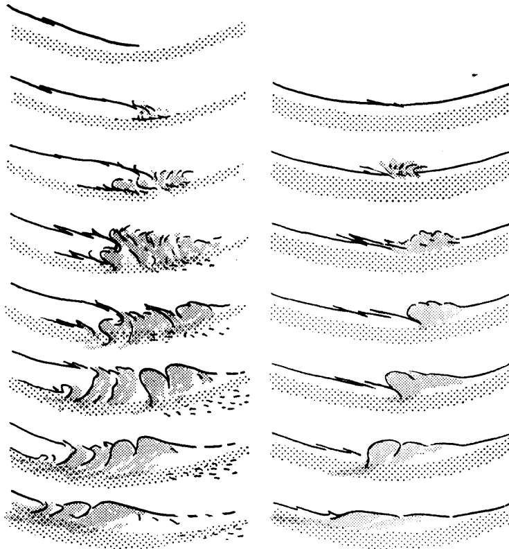
Fig. 5. Development of electron aurora and hydrogen emission during a local breakup which occurred in the evening of May 17, 1971. Though the pattern of the activity is much smaller than the previous examples, the general feature of development closely resembles the latter.
