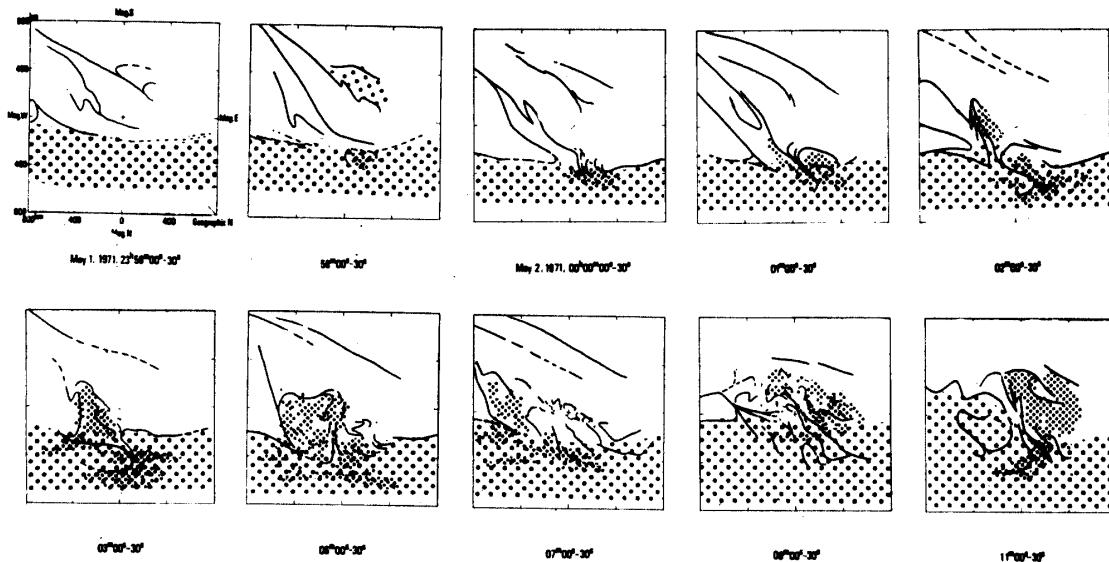
(2c) Linear scale representation of the pattern and the development of electron aurora and hydrogen emissions.
