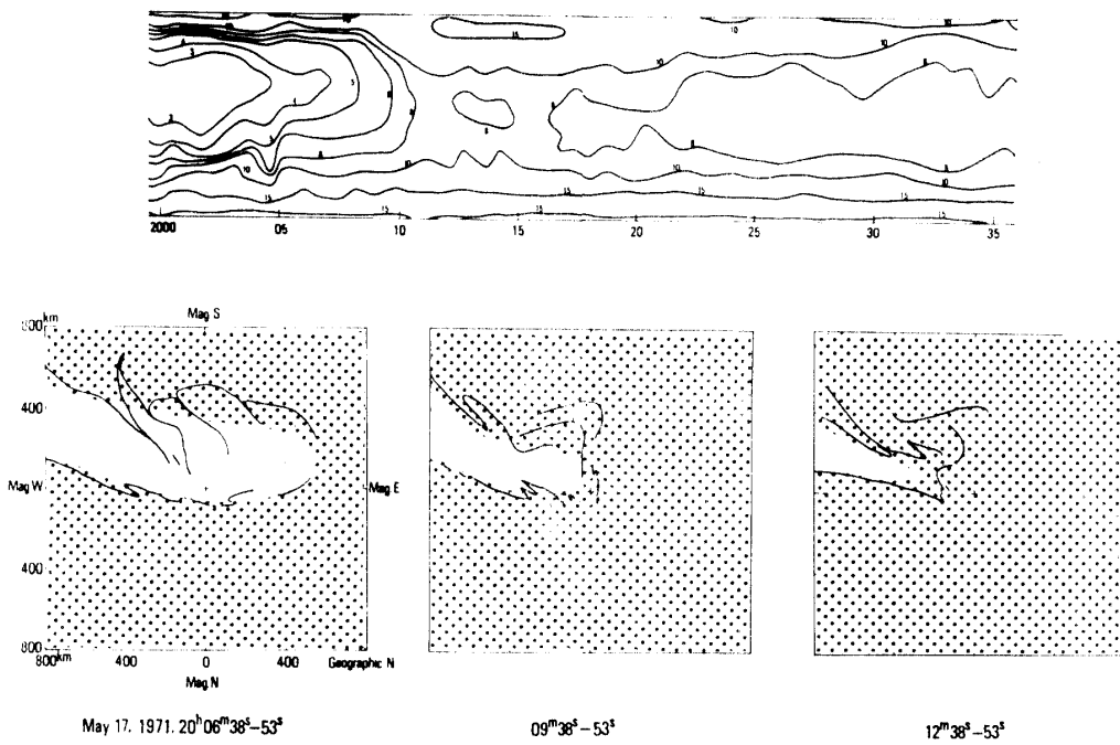
Fig. 4. Westward drift of the electron auroral arc (loop), immediately followed by that of the hydrogen emission region, during the auroral breakup of May 17, 1971. Dotted area is a schematic illustration of the hydrogen region.
