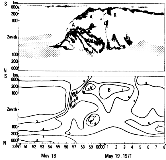
(1b) Top: Meridian-time display of the electron aurora. Dense and sparse dots indicate active and diffuse auroras, respectively. Bottom: Meridian-time display of hydrogen ( H_{\beta} ) emission. The unit of the intensity contours is Rayleigh/Å.
