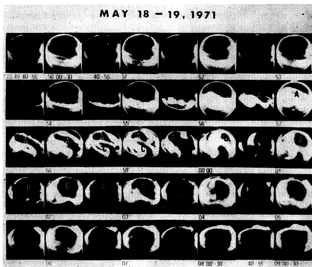
(1a) All-sky camera photographs (in local geomagnetic coordinate; top-south, left-west).
