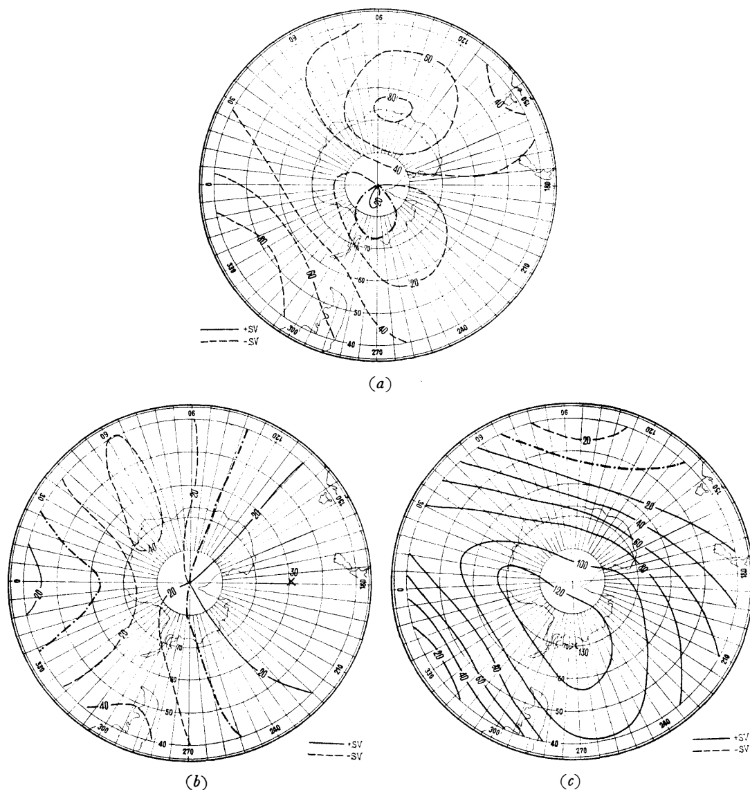
Fig. 2 Isoporic charts of the Antarctic ( \delta X 1959-1964).
