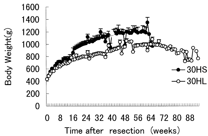
Fig. 1 A comparison of body weight changes between the 30HS and 30HL groups. All values are expressed as means \pm SEM.
