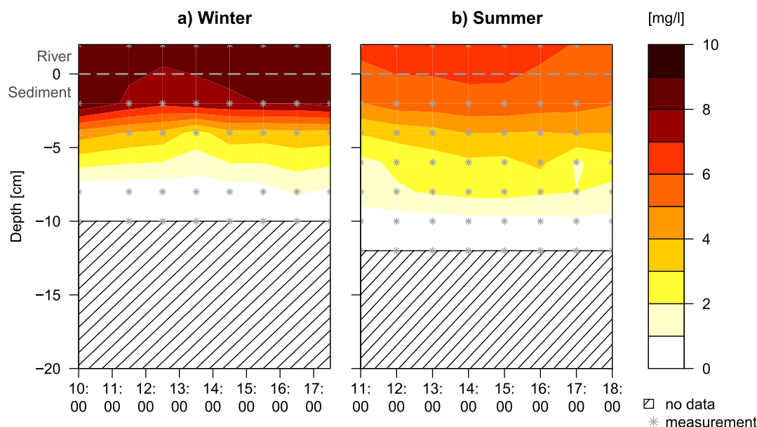
Figure 3. Time series of oxygen depth profiles and time in winter and summer.
