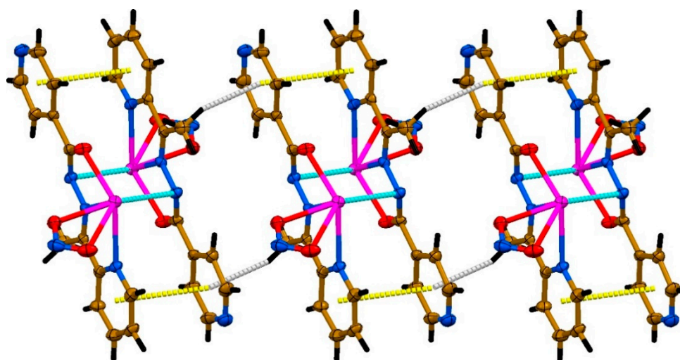
Figure 2. View on a 1D supramolecular chain in the structure of [\text{PbL}(\text{NO}_2)]_n , formed through \text{Pb}\cdots\text{N}=\text{C}(\text{O}) tetrel bonds, \pi\cdots\pi stacking, and \text{C}-\text{H}\cdots\pi interactions (ellipsoids are drawn at 50% probability level). Color code: H = black, C = gold, N = blue, O = red, and Pb = magenta; cyan dashed line = \text{Pb}\cdots\text{N} tetrel bond, yellow dashed line = \pi\cdots\pi stacking interaction, and gray dashed line = \text{C}-\text{H}\cdots\pi interaction.
