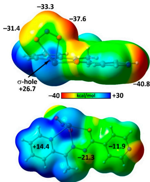
Figure 5. Two views of the molecular electrostatic potential (MEP) surface of [\text{PbL}(\text{NO}_2)]_n (isosurface 0.001 a.u.). The blue color is used for positive MEP values, and the red color for negative values, as indicated in the legend.
