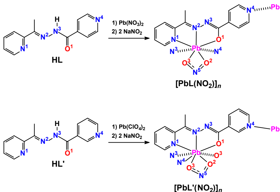
Scheme 1. Syntheses of [\text{PbL}(\text{NO}_2)]_n (this work) and [\text{PbL}'(\text{NO}_2)]_n [37] (tetrel bonds shown as dashed lines).
