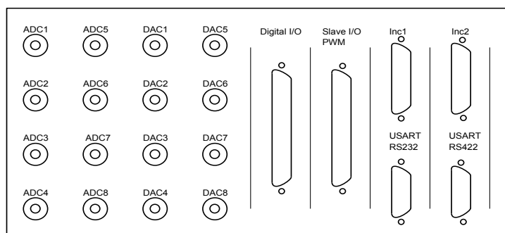
Fig. 5.4: CP1104 connection panel.
