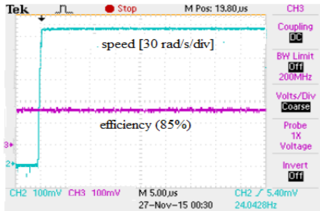
Fig. 5.6: Experimental speed and efficiency responses of the proposed DTFC at rated speed and 50% rated load.
