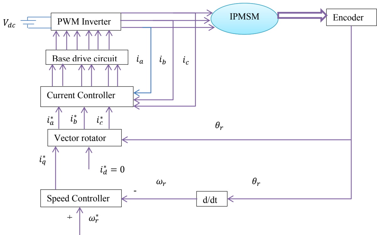
Fig. 1.5: Block diagram of the vector control scheme of the IPMSM drive.
