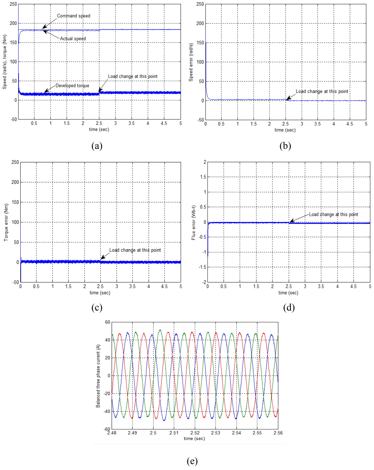
Fig.6.25: Simulated response of the proposed nonlinear controller at rated speed with step change of load (15-19 Nm): (a) speed and developed torque; (b) speed error; (c) torque error; (d) flux error; (e) balanced three phase current.
