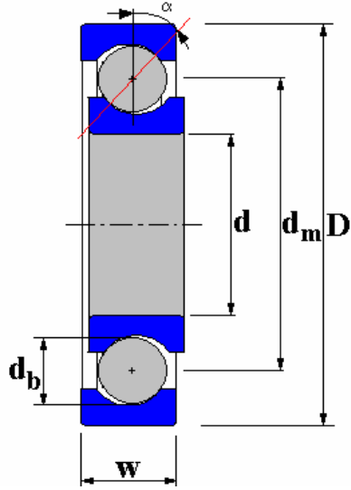
Figure 2.2. Geometry of ball bearing [33].
