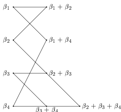
FIGURE 2: The digraph G_{\mathfrak{M}} (simplified form).
