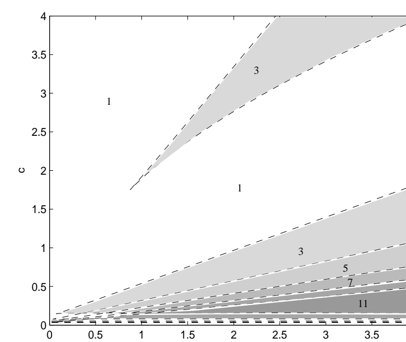
Values indicate the number of roots for \Lambda = 0.5 . The shaded areas show where there is more than one branch of linear waves.
