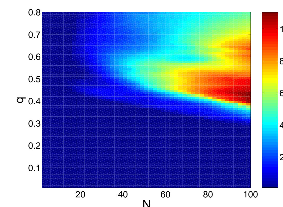
Minimum value of the amplitude at the collision point after the collision as a function of the norm and the momentum. We have supposed that the trapped energy in the regime is zero in order to clarify the figure.
