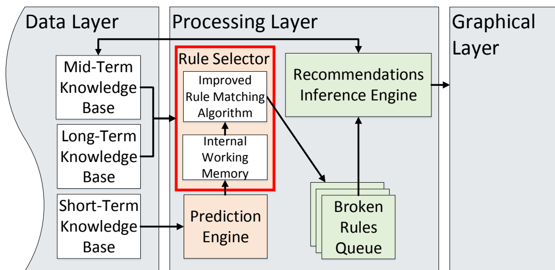
Figure 5.1: The data flow of the processing layer with the focus on the rule selector module and its local working memory and improved rule matching algorithm
