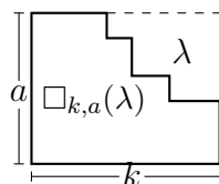
Figure 1: The partition \square_{k,a}(\lambda)
