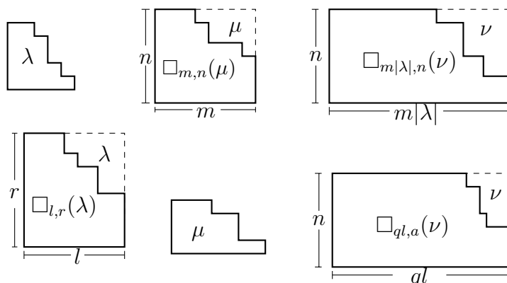
Figure 3: The partitions in the symmetry of Theorem 12 or Equation (6) (top) and Theorem 14 or Equation (8) (bottom)
