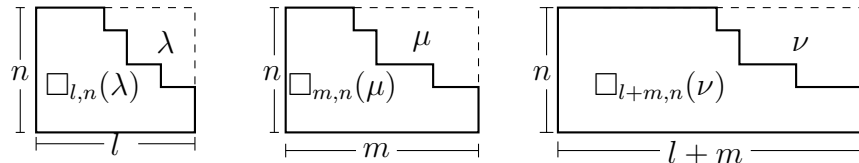
Figure 2: The partitions occurring in the symmetry of Theorem 4
