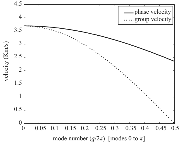
Fig. 4. Phase and group velocities in the Coulomb's chain, both give at q \rightarrow 0 the sound velocity, which can be compared with the values of 3.4-3.7 km/s obtained in Ref. [12].
