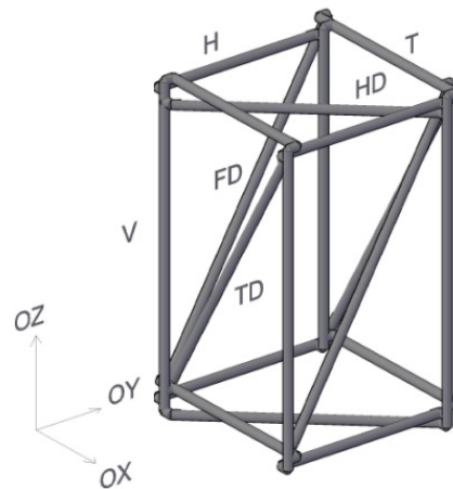
Figure 1. Prismatic module, OX = 1'00m , OY = Variable , OZ = 1'70 m .
