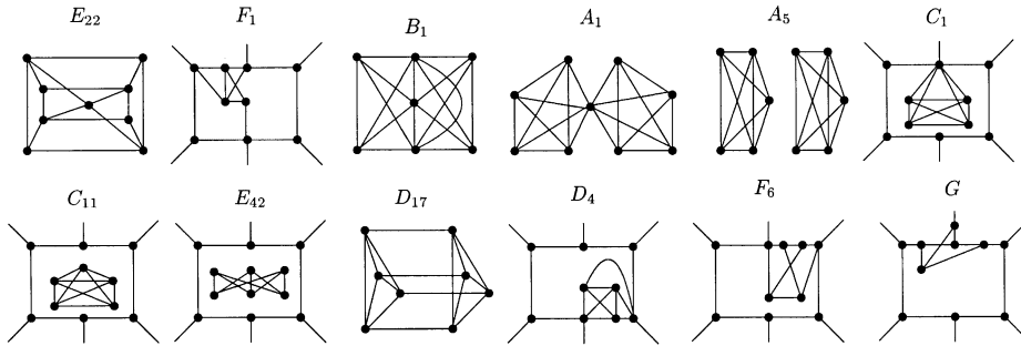
Fig. 11. Twelve forbidden minors for the projective plane.
