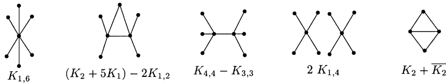
Fig. 9. List \mathcal{L} of forbidden topological minors for a projective total graph.
