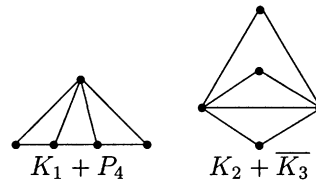
Fig. 4. K_1 + P_4 and K_2 + \overline{K_3} .
