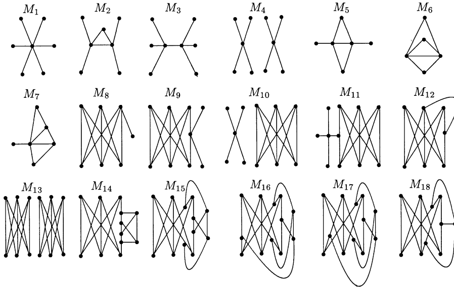
Fig. 15. List \mathcal{D} of graphs with a non-projective middle graph.
