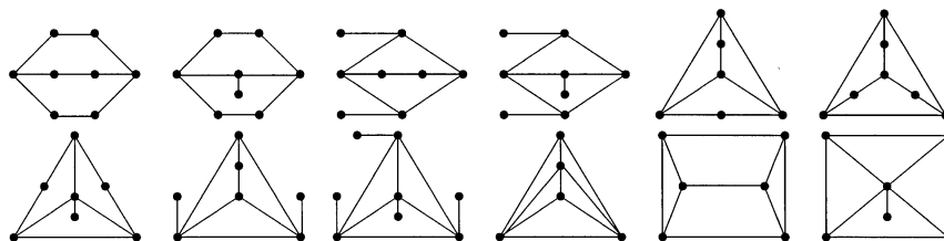
Fig. 1. Sedláček's list of forbidden generalized outerplanar subgraphs.
