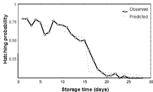
Fig. 4: Piecewise regression fit for hatching probability as a function of the storage time of the eggs
