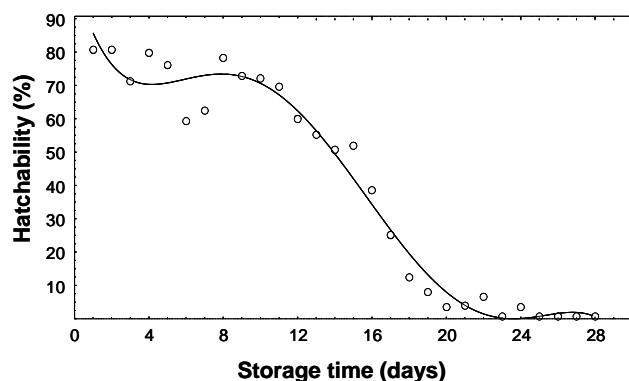
Fig. 1: Fifth-degree polynomial fit for hatchability as a function of the storage time of the eggs
