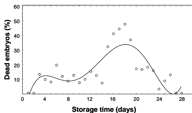
Fig. 2: Fifth-degree polynomial fit for dead embryos as a function of the storage time of the eggs
