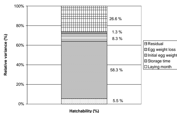
Fig. 5: Relative components of the variance for the effects of laying month, storage time, initial egg weight, egg weight loss after 39 days of incubation on the variability of hatchability (%)
