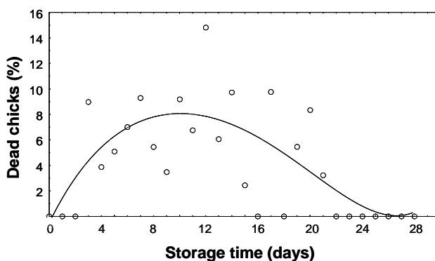
Fig. 3: Fifth-degree polynomial fit for dead chicks as a function of the storage time of the eggs
