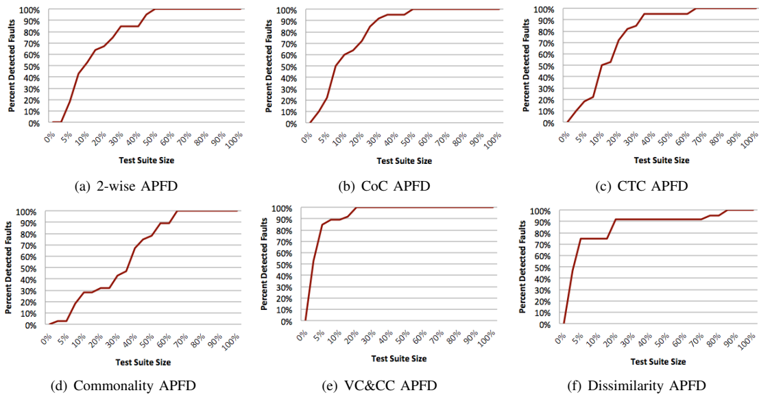
Fig. 4: APFD metrics for Random3 model
