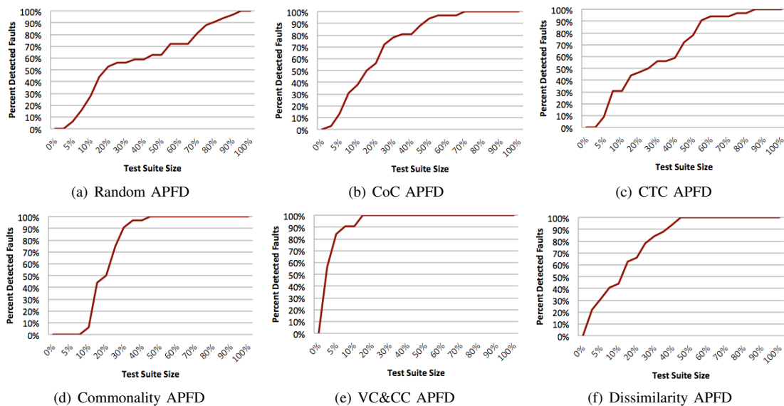
Fig. 3: APFD metrics for Random3 model
