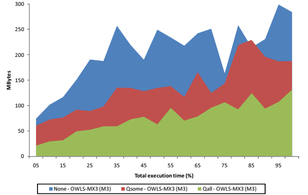
Figure 4: Memory consumption statistics when filtering OWLS-MX3 (M3).
