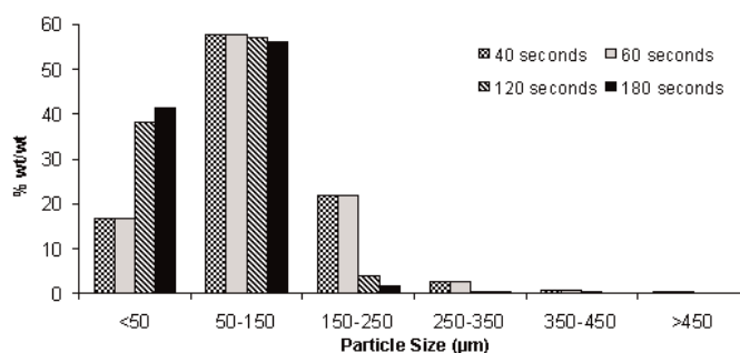
Figure 1. Particle size distribution after several crushing times.
