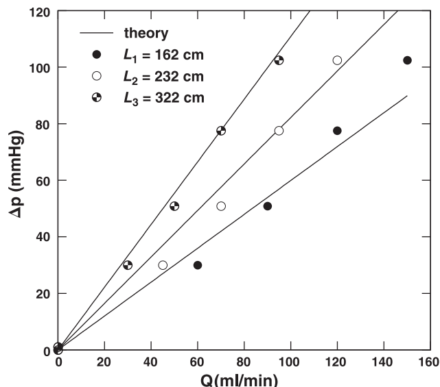
Fig. 5. Experimental pressure drop along the three vessels (of length L ) associated in parallel as a function of the flow rate. The solid line corresponds to the pressure drop according to the theory, which includes the pressure drop due to viscous losses (Poiseuille's law) and the local pressure drop due to the presence of the flowmeter.
