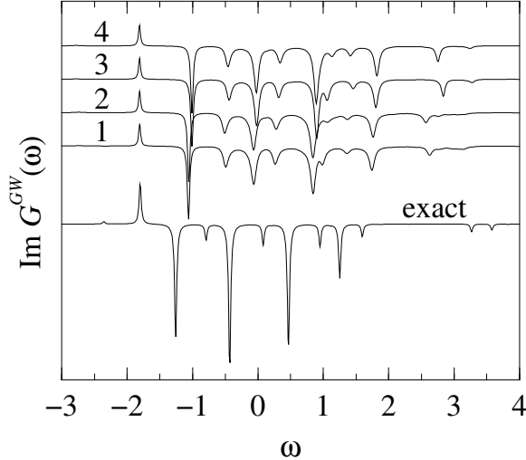
Figure 4: Using a renormalized Green’s function or screening in the GW self-energy without vertex corrections fails to improve the spectrum. The numbered curves indicate the combinations (1) G^0W^{\text{RPA}}[G^0] , (2) GW^{\text{RPA}}[G^0] , (3) G^0W^{\text{RPA}}[G] and (4) GW^{\text{RPA}}[G] for two electrons on a twelve-site chain with U = 2 .
