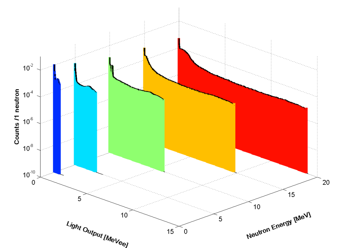
Figure 11: Detector Response Matrix Simulation (NE-213)
