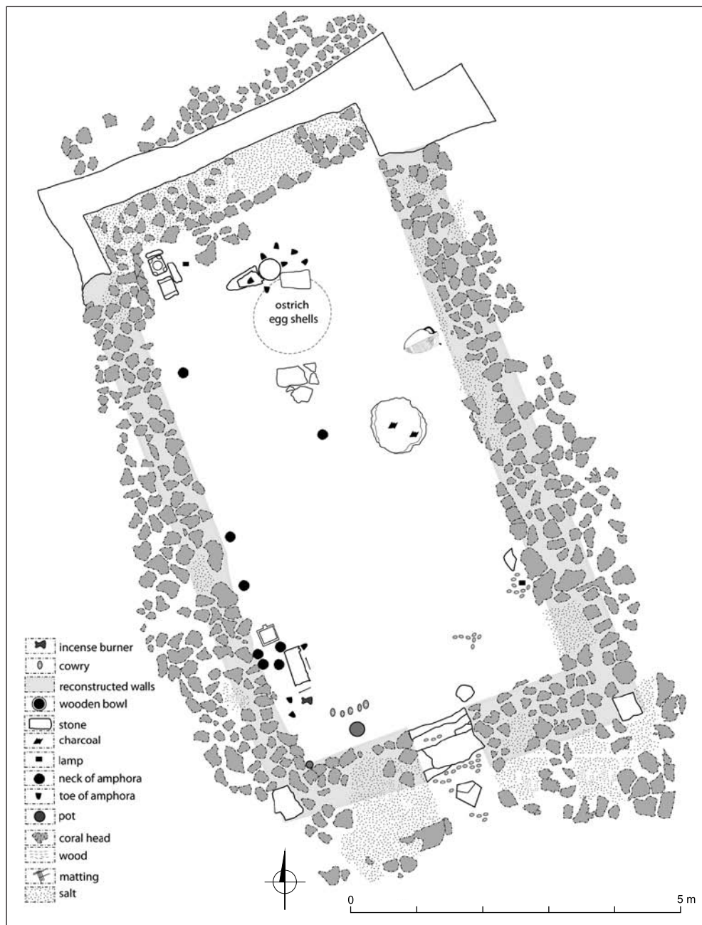
Fig. 8A. Plan of the harbor temple in the latest occupational phase (5th century) (Drawing J. Rądkowska; digitizing S. Maślak and U. Wicenciak)
