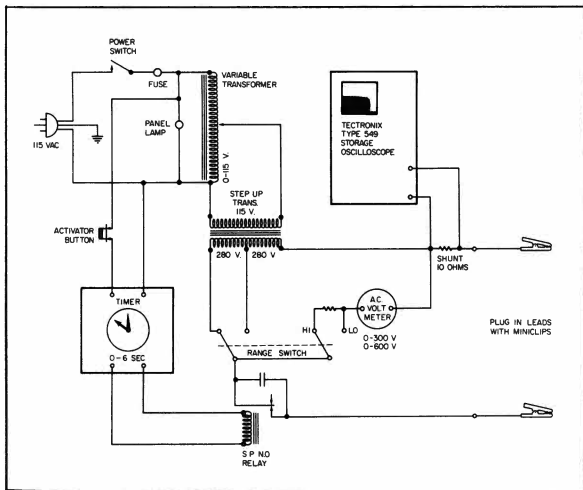
Fig. 7—Wiring diagram of experimental apparatus.
