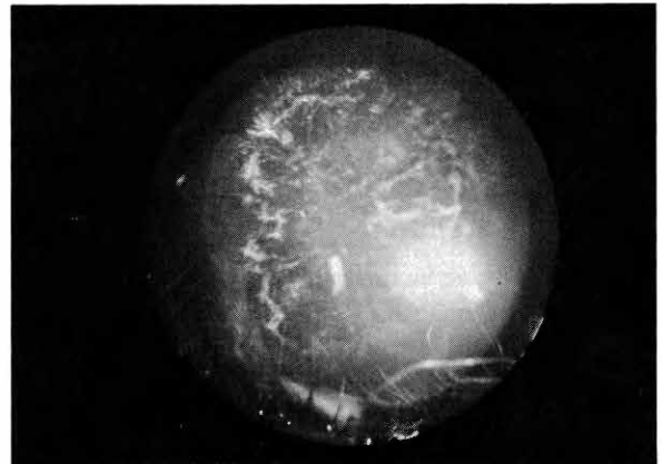
Fig. 5—Cataracta electrica in animal receiving 26.51 watt-seconds.
