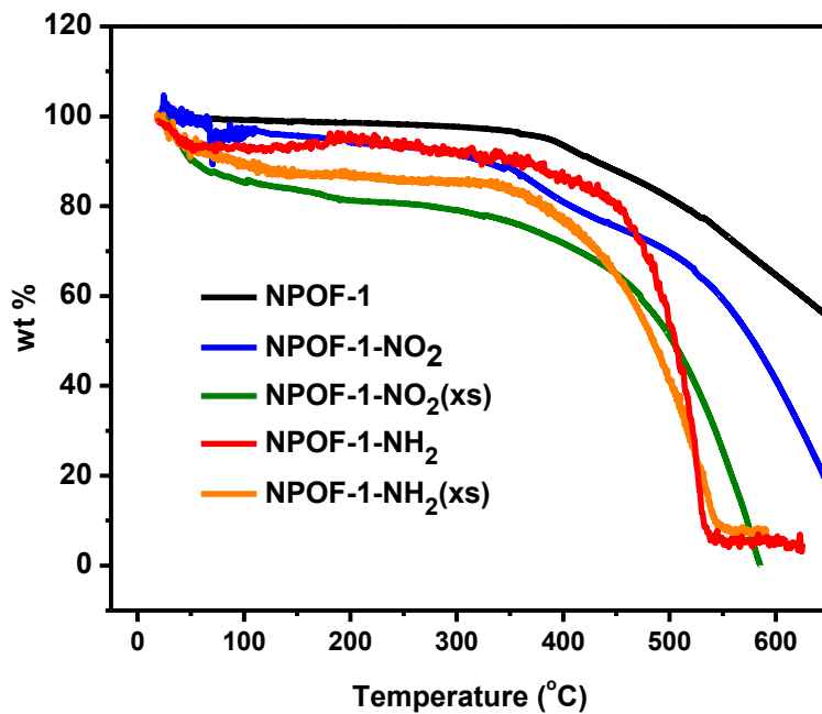
Figure 3.3. TGA traces of polymers.
