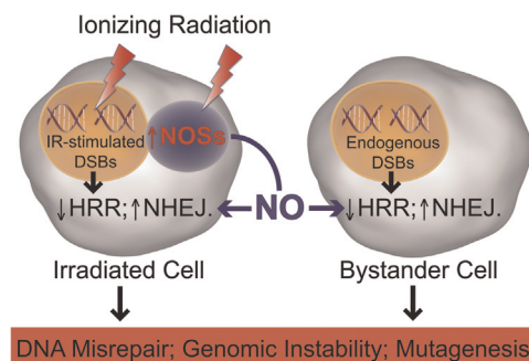
Fig. 2. Activation of NOSs in irradiated cells leads to NO-dependent downregulation of HRR/NHEJ ratio with subsequent maintenance of genomic instability in both irradiated and bystander cells.
