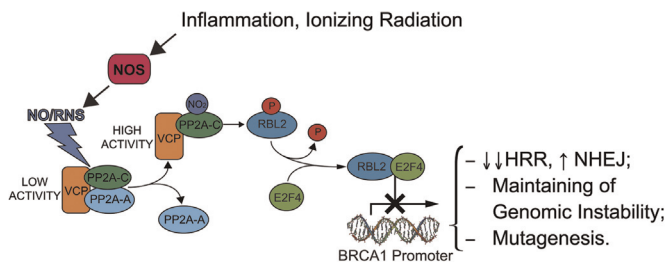
Fig. 1. Schematic representation of NO/RNS-dependent stimulation of genomic instability.
