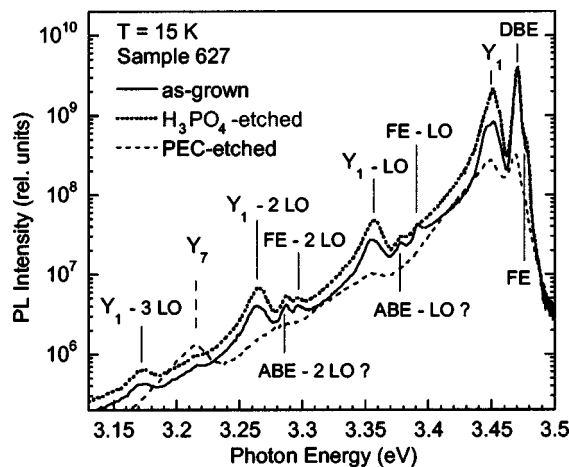
FIG. 94. Low-temperature PL spectrum of the N-polar GaN layer grown by MBE on sapphire substrate, P_{exc}=300 W/cm^2 . A piece of the sample was etched in H_3PO_4 at 100 °C for 10 s and another piece of the sample was etched by PEC method.
