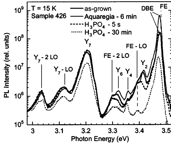
FIG. 93. Effect of etching of Ga-polar GaN in boiled aqua regia for 6 min and in H_3PO_4 at 160 °C for 5 s and 30 min. P_{exc}=100 W/cm^2 . See the surface morphologies for this sample in Fig. 92.
