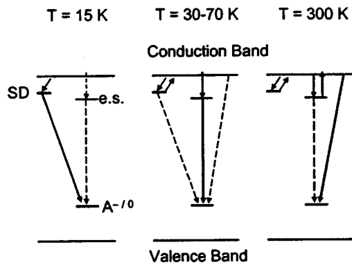
FIG. 34. Schematic of transitions responsible for the GL band in high-purity GaN. e.s. is the excited state of the acceptor, therefore the transition e.s. \rightarrow A^{-1/0} is of intracenter type. SD stands for the shallow donors, and the transitions involved are distant DAP transitions. The dashed lines correspond to less probable transitions, whereas the solid lines show the dominant transitions.
