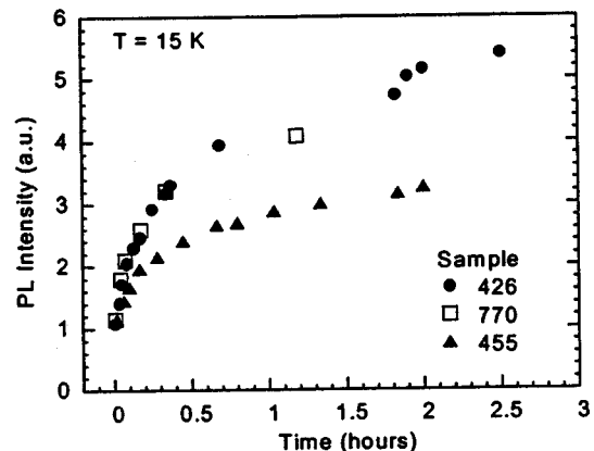
FIG. 96. Evolution of PL intensity at 3.36 eV with time of HeCd laser exposure. T=15 K. P_{exc}=200 W/cm^2 .
