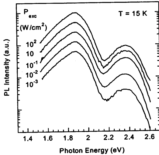
FIG. 49. Effect of excitation density, P_{exc} , on low-temperature PL spectrum of the Ga-rich GaN layer. Position and shape of the bands are independent of excitation density with accuracy of \pm (5-10) meV. The curves are shifted arbitrarily in the vertical direction (log scale).
