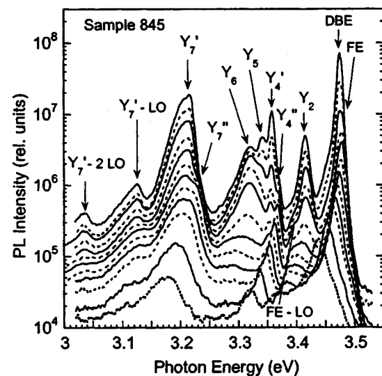
FIG. 100. Temperature dependence of PL spectrum at P_{exc} = 100 W/cm 2 for as-grown Ga-polar GaN layer by MBE on top of the HVPE-grown 10- \mu m-thick GaN on sapphire substrate. Temperatures are 15, 35, 60, 100, 140, 195 K (solid curves), 25, 50, 80, 120, 160 K (dashed curves), and 240 K (dotted curve). Reprinted with permission from Reshchikov et al. , Mater. Res. Soc. Symp. Proc. 693, I6.28 (2002).
