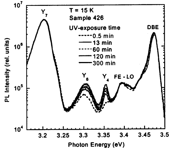
FIG. 95. Transformation of PL spectrum with time of exposure by HeCd laser at 15 K. P_{exc}=200 W/cm^2 . The sample was etched in H_3PO_4 at 160 °C for 1 min and subsequently exposed to air for 20 days. Reprinted with permission from Reshchikov et al. , Mater. Res. Soc. Symp. Proc. 743, L11.3 (2003).
