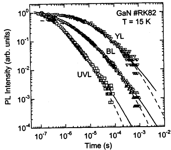
FIG. 17. Intensity of the YL, BL, and UVL bands at 15 K in undoped GaN grown by MOCVD. The curves are calculated using Eq. (17). Reprinted with permission from Korotkov et al. , Physica B 273, 80 (1999). Copyright (1999) by Elsevier.
