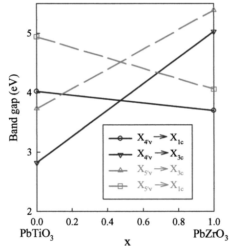
FIG. 9. Calculated band-gap energies of PZT as a function of Zr composition. The lines assume linear interpolation between the two end-point compounds, \text{PbTiO}_3 and \text{PbZrO}_3 .
