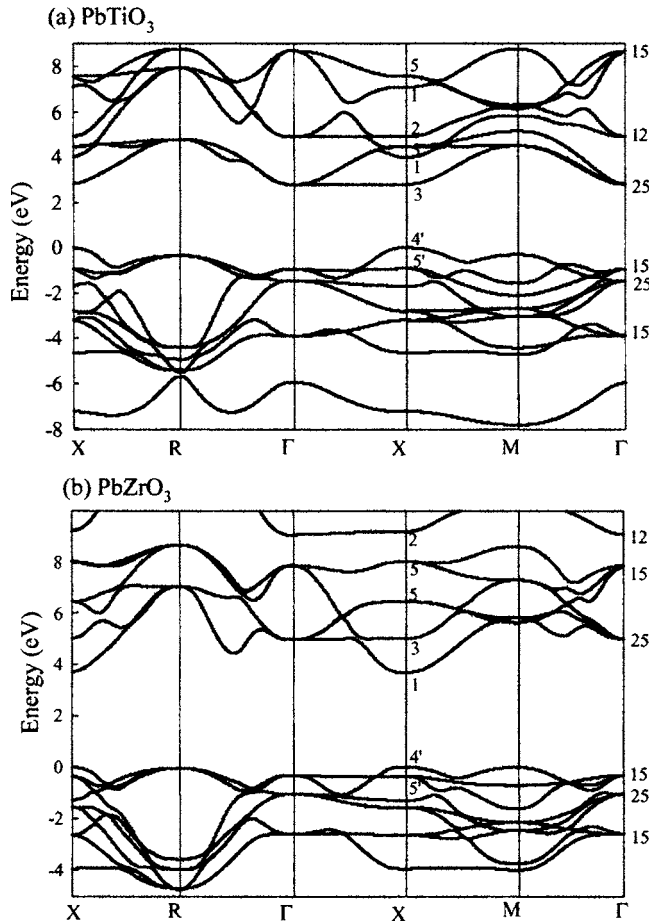
FIG. 8. Calculated band structure of (a) \text{PbTiO}_3 and (b) \text{PbZrO}_3 . The energy zero is at the top of the valence band.
