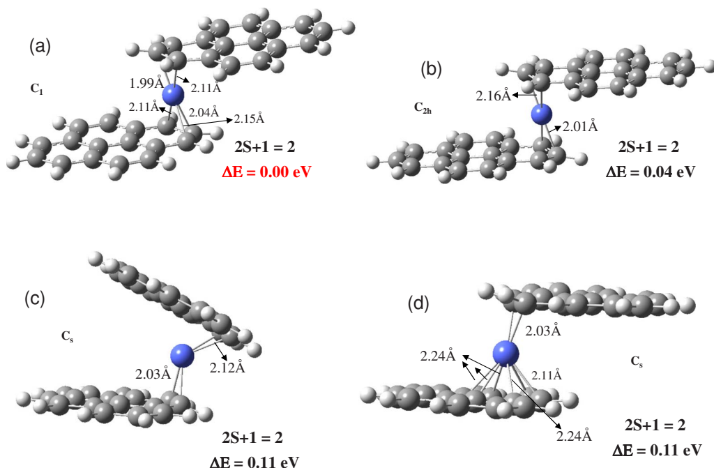
FIG. 10. (Color online) The ground state and higher energy isomers of the neutral \text{Co}(\text{pyrene})_2 complex.
