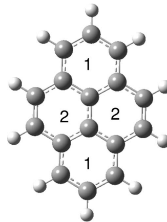
FIG. 1. Pyrene ( \text{C}_{16}\text{H}_{10} ) molecule. The two different carbon rings are identified.
