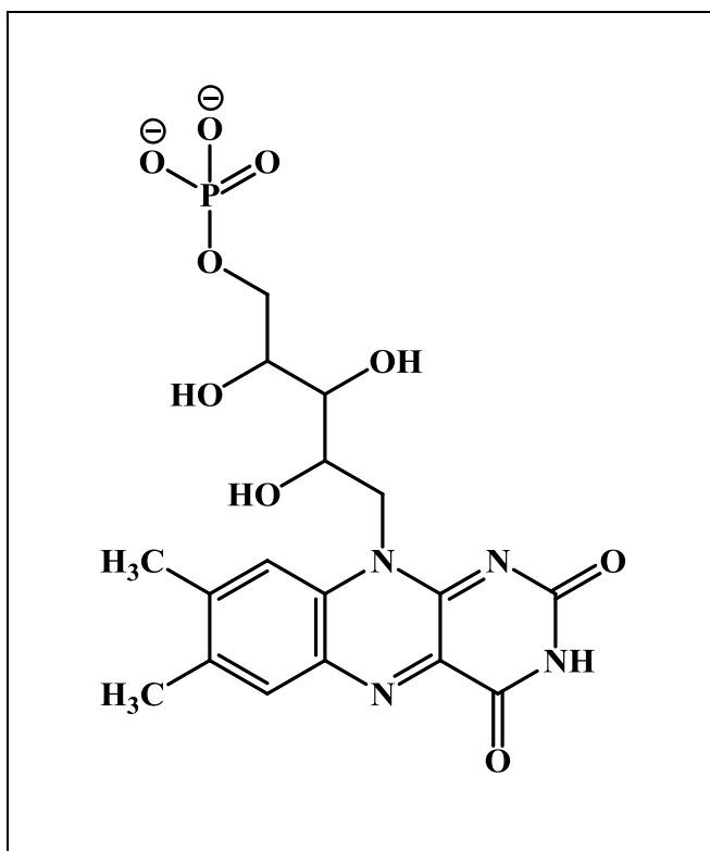
Figure 14: Structure of flavin mononucleotide (FMN)
