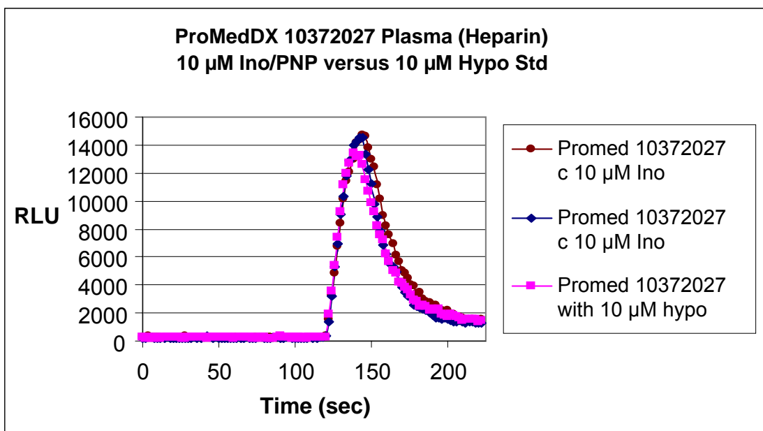
Figure 26. Charts depicting inosine and PNP incubation time and conversion study. Evaluation of 60 and 120 sec PNP incubation times, with 120 sec demonstrating the complete conversion of inosine to hypoxanthine. The 10 \mu M inosine with PNP conversion RLU responses (n=2) overlays completely against the 10 \mu M hypoxanthine standard.
