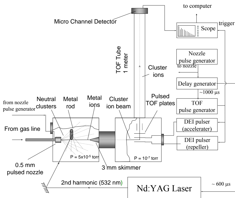
Figure 2: Experimental setup of Time-of-flight mass spectrometer (TOFMS) for the generation of metal cation – containing molecular clusters.
