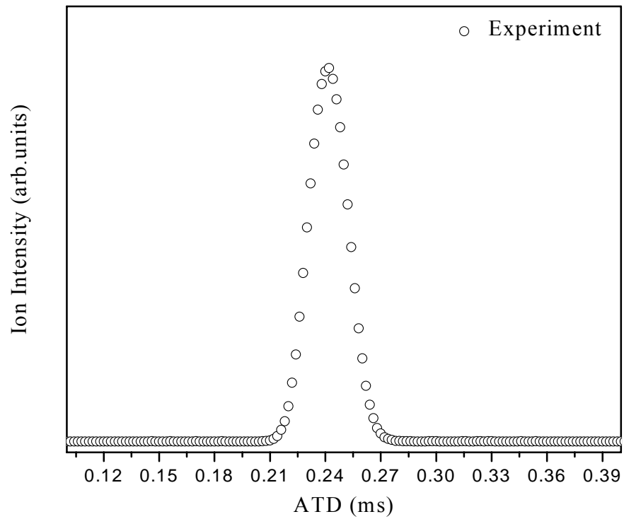
Figure 80: Arrival time distribution of Mg + ions, produced from LVI process. The experimental conditions are: 5 \mu s gate width, drift cell pressure (He) = 2.497 torr, drift cell temperature at 298.25 K and 42 V voltage difference across the cell
