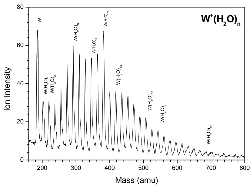
Figure 112: TOF mass spectra of \text{W}^+(\text{H}_2\text{O})_n
