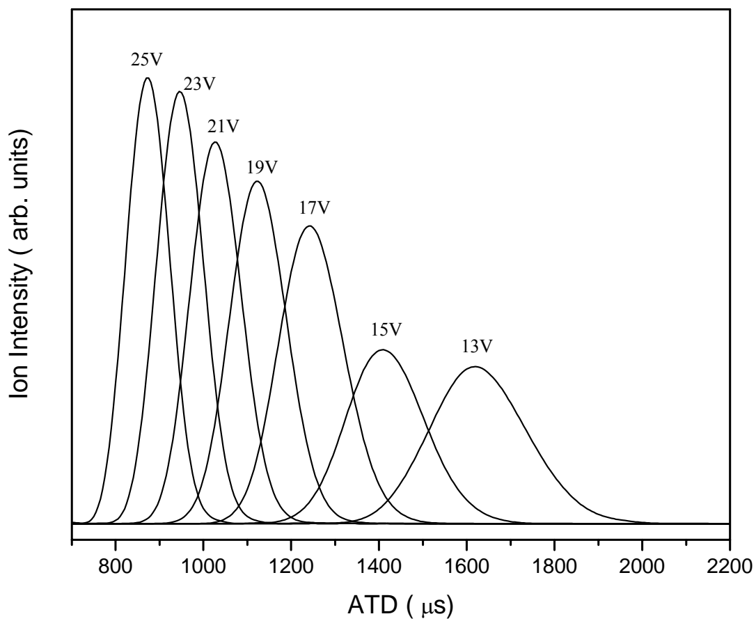
Figure 8: Arrival time distribution of mass selected C_8H_8^+ ions at different cell voltages : Experimental conditions are: 50 \mu s pulse width, injection energy is 15 eV, 2.007 Torr and the drift cell temperature is 27.3 ^{\circ}C .
