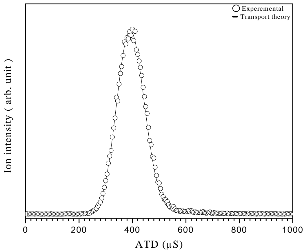
Figure 49: Arrival time distribution of mass selected (C_8H_8)_2^+ (formed by EI of the continuous flow of the heated styrene and AIBN vapors at T = 92.3 °C)(circles) and the predicted distribution from transport theory (solid line). Experimental conditions are: the source temperature is 92.3 °C, 50 \mu s pulse width, injection energy is 14 eV, 1.682 Torr He inside the drift cell, the drift cell temperature is 29.65 °C 25 V voltage difference between the entrance and the exit lenses. The measured reduced mobility K_0 = 5.82 cm^2V^{-1}s^{-1} .
