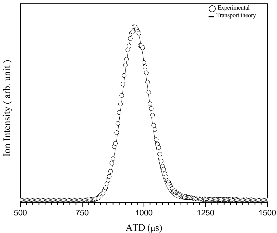
Figure 32: Arrival time distribution of (\text{C}_8\text{H}_8)_2^+ ions at drift cell temperature of 373 K (circles) and the predicted distribution from transport theory (solid line). Experimental conditions are: 50 \mu\text{s} pulse width, injection energy is 15 eV, 1.278 Torr He inside the drift cell, the drift cell temperature is 99.70 ^\circ\text{C} 18 V voltage difference between the entrance and the exit lenses and E/N = 6.12 Td. The reduced mobility K_0 = 5.34 \text{ cm}^2\text{V}^{-1}\text{s}^{-1} .
