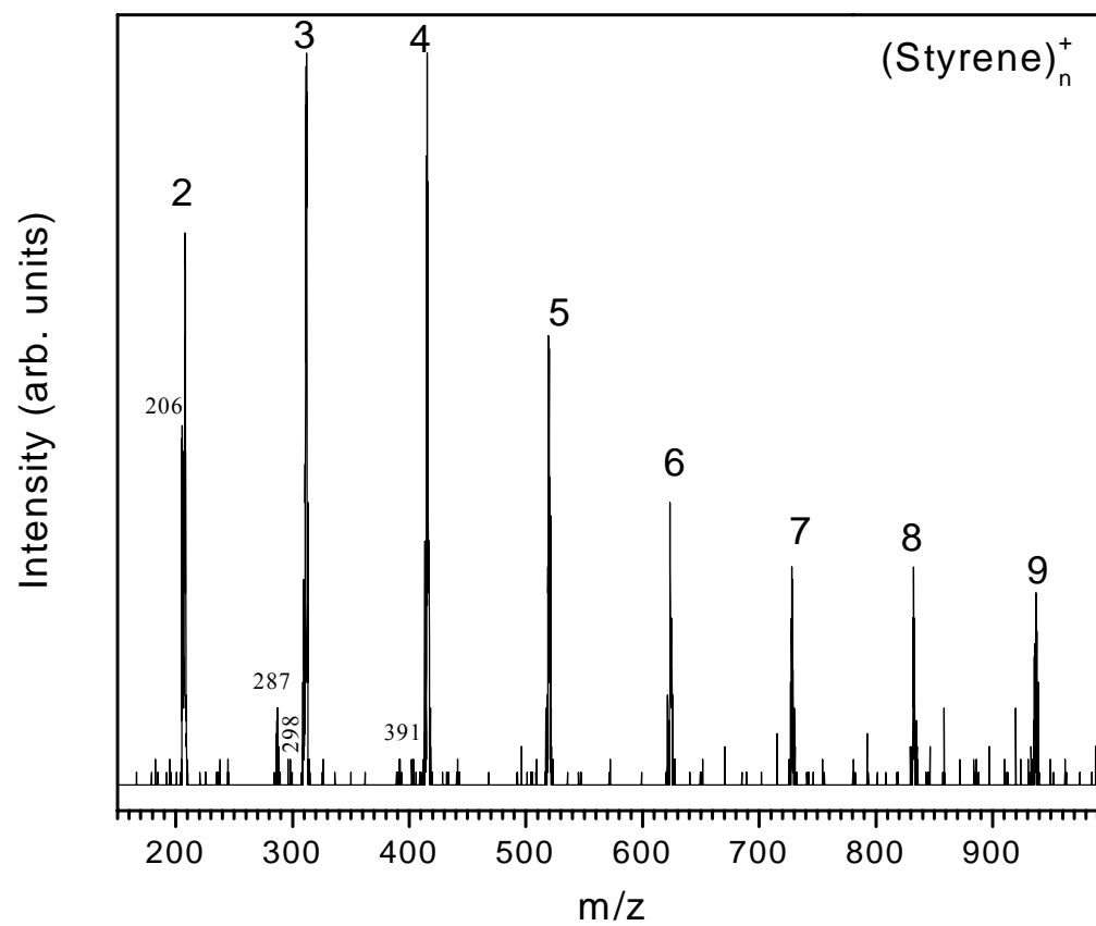
Figure 12: Mass Spectrum of (\text{C}_8\text{H}_8)_n^+ clusters ions produced by 90 eV Electron Impact ionization, and then injected into 1.159 Torr He with 15 eV injection energy.
