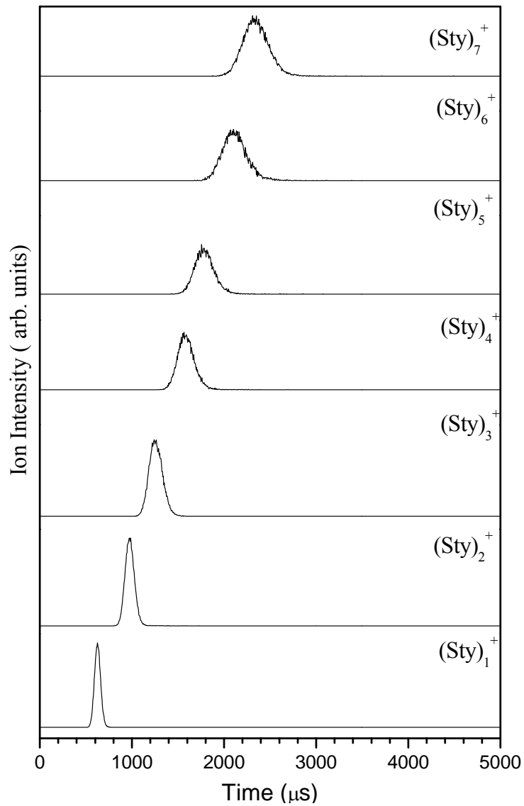
Figure 23 : The measured Arrival time distribution of (\text{C}_8\text{H}_8)_n^+ ions, with n = 1-7 with same E/N = 6.23 \text{ 0.1} .
