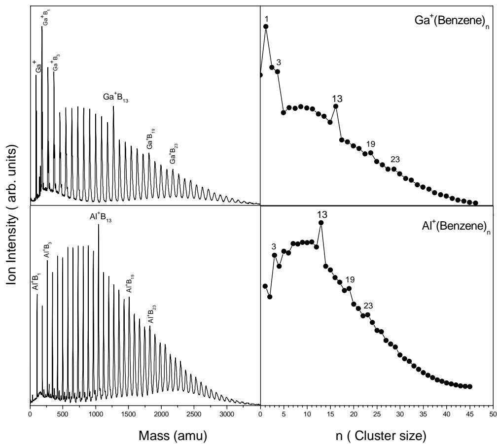
Figure 65: TOF mass spectra and ion intensity distribution as a function of cluster size of \text{M}^+(\text{Benzene})_n where \text{M} = \text{Al} and \text{Ga} .
