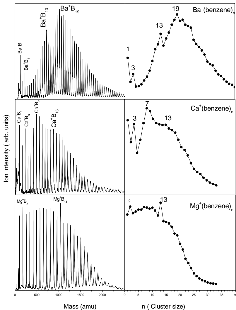
Figure 64: TOF mass spectra and ion intensity distribution as a function of cluster size of M^+ (Benzene) n where M = \text{Mg, Ca and Ba} .
