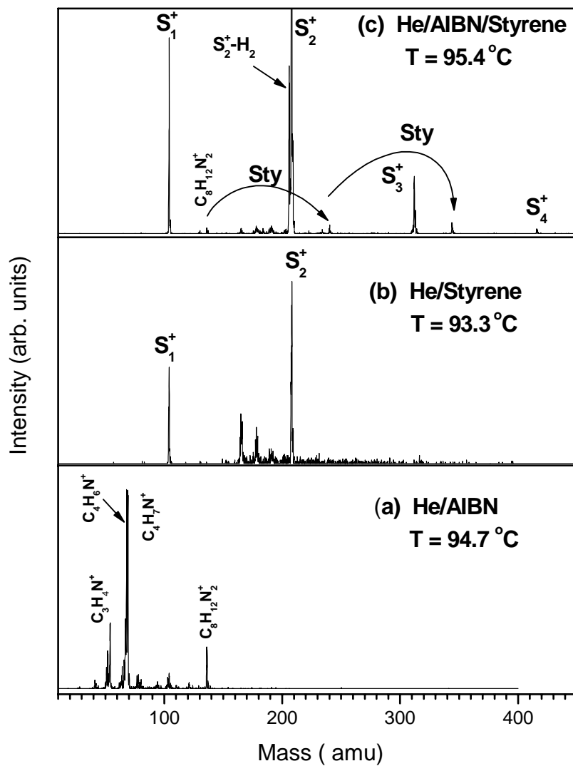
Figure 48: Mass spectra when the source contained: (a) only the initiator AIBN (2,2'-Azo-bis- iso butyronitrile ( \text{C}_8\text{H}_{12}\text{N}_4 )) at T = 94.7\text{ }^{\circ}\text{C} ; (b) only styrene vapor at T = 93.3\text{ }^{\circ}\text{C} and (c) styrene + AIBN at T = 95.4\text{ }^{\circ}\text{C} .
