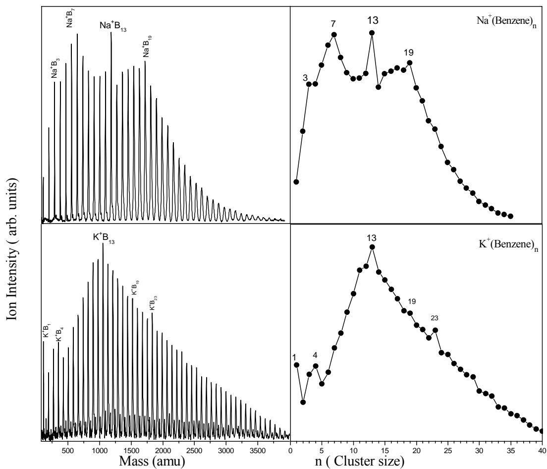
Figure 63: TOF mass spectra and ion intensity distribution as a function of cluster size of M^+(\text{Benzene})_n where M = \text{Na} and \text{K} .
