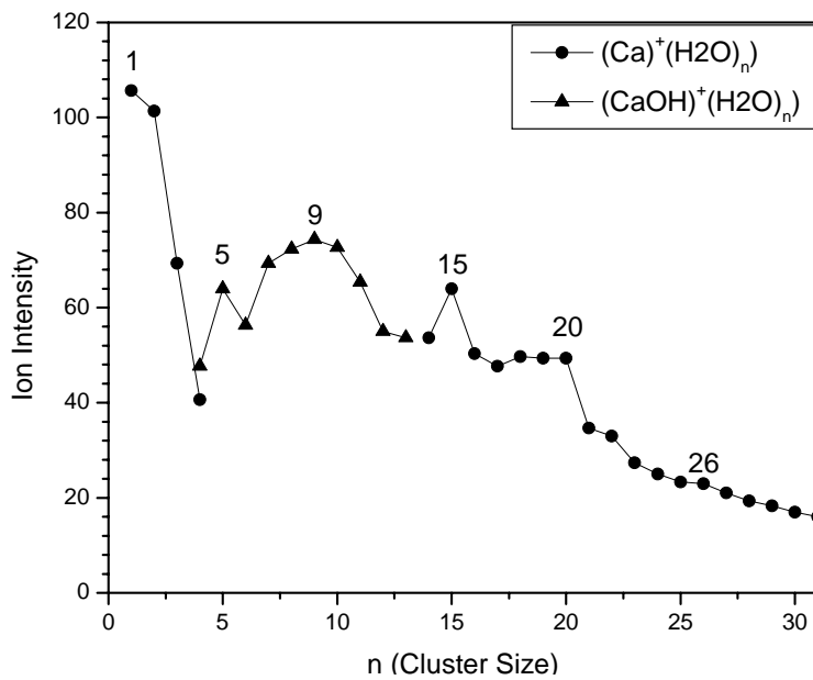
Figure 97: \text{Ca}^+(\text{H}_2\text{O})_n ion intensity distribution as a function of cluster size
