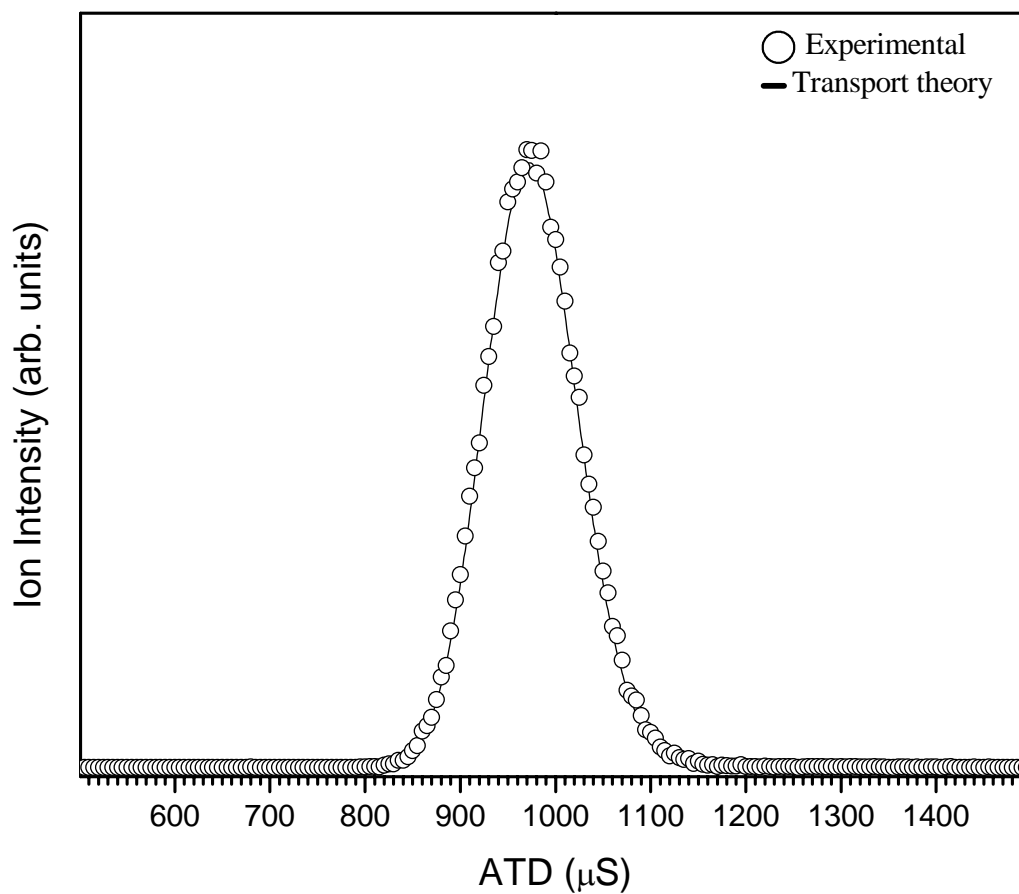
Figure 22: Arrival time distribution of mass selected (C_8H_8)_2^+ ions (circles) and the predicted distribution from transport theory (solid line). Experimental conditions are : 50 \mu s pulse width, injection energy is 15 eV, 1.136 Torr He inside the drift cell, cell temperature is 31.9 ^{\circ}C , 25 V the voltage difference between the entrance and the exit lenses and E/N = 6.26 Td. The reduced mobility K_0 = 5.86 cm^2V^{-1}s^{-1} .
