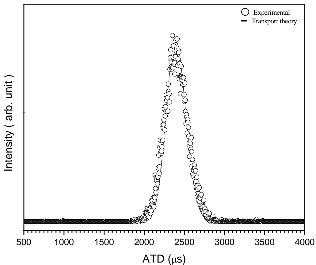
Figure 30: Arrival time distribution of (C_8H_8)_8^+ ions (circles) and the predicted distribution from transport theory (solid line). Experimental conditions are: 50 \mu s pulse width, injection energy is 15 eV, 1.152 Torr He inside the drift cell, the drift cell temperature is 28.6^\circ C , 25 V voltage difference between the entrance and the exit lenses and E/N = 6.10 Td. The reduced mobility K_o = 2.28 \text{ cm}^2\text{V}^{-1}\text{s}^{-1} .
