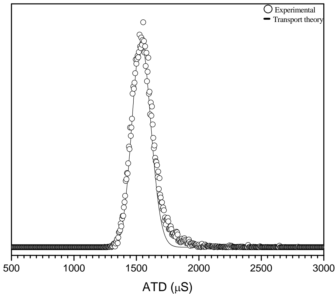
Figure 26: Arrival time distribution of mass selected (C_8H_8)_4^+ ions (circles) and the predicted distribution from transport theory (solid line). Experimental conditions are: 50 \mu s pulse width, injection energy is 15 eV, 1.098 Torr He inside the drift cell, the drift cell temperature is 30.80 ^{\circ}C , 20 V voltage difference between the entrance and the exit lenses and E/N = 6.45 Td. The reduced mobility K_0 = 3.55 cm^2V^{-1}s^{-1} .
