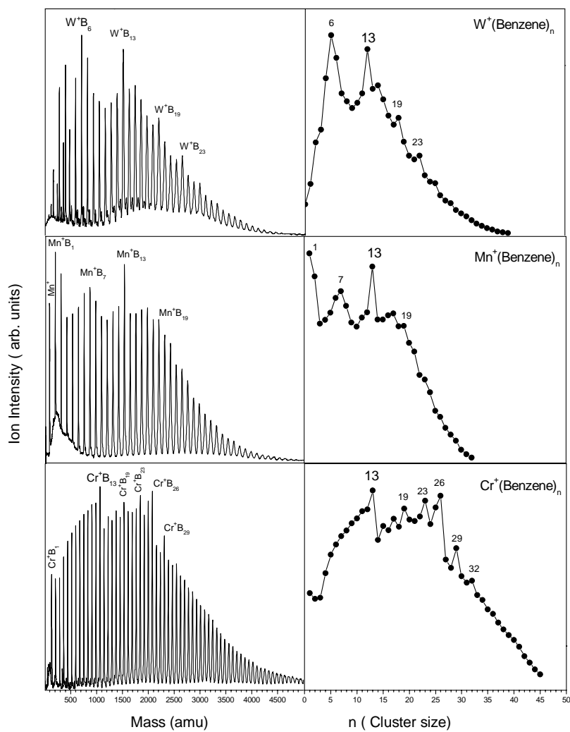
Figure 66: Mass spectra and ion intensity distribution as a function of cluster size of M^+ (Benzene)_n where M = Cr, Mn and W .
