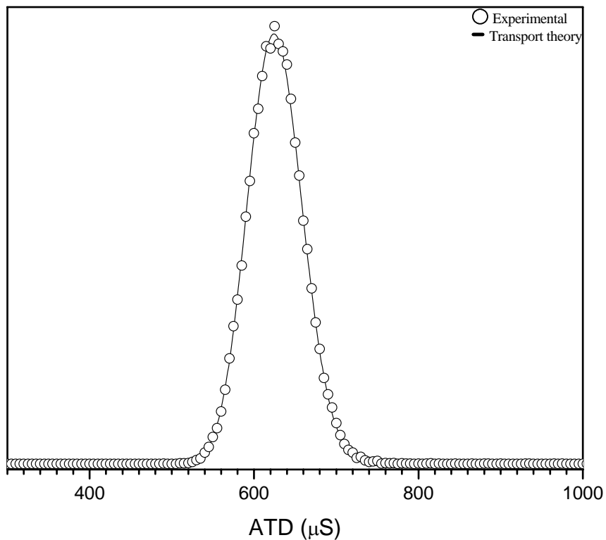
Figure 10: Arrival time distribution of mass selected C_8H_8^+ ions (circles) and the predicted distribution from transport theory (solid line): Experimental conditions are : 50 \mu s pulse width, injection energy is 15 eV, 1.136 Torr He inside the drift cell, 20 V voltage cell temperature is 31.7 ^{\circ}C , difference between the entrance and the exit lenses and E/N = 4.01 Td. The reduced mobility K_0 = 9.28 cm^2V^{-1}s^{-1} .
