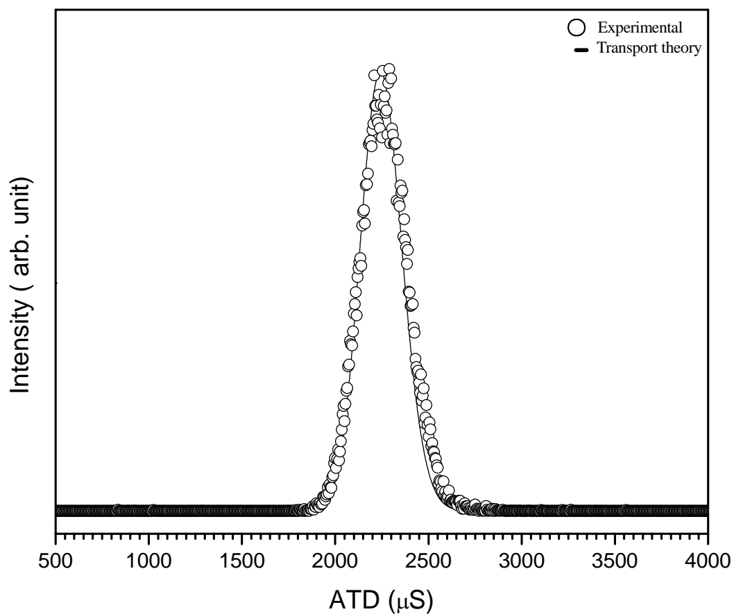
Figure 29: Arrival time distribution of (C_8H_8)_7^+ ions (circles) and the predicted distribution from transport theory (solid line). Experimental conditions are: 50 \mu s pulse width, injection energy is 15 eV, 1.152 Torr He inside the drift cell, the drift cell temperature is 28.6 ^{\circ} C 20 V voltage difference between the entrance and the exit lenses and E/N = 4.88 Td. The reduced mobility K_0 = 2.50 cm^2V^{-1}s^{-1} .
