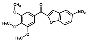
CTR 105
