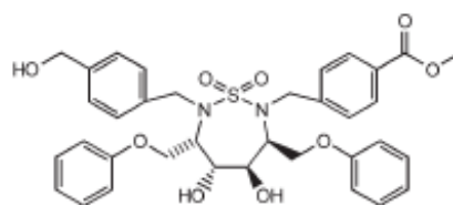
Aha024 (1G35)
