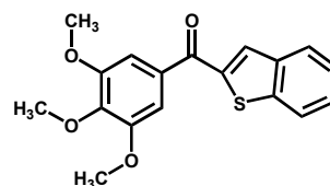
CTR 104
