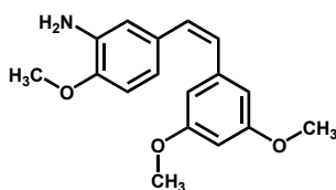
Stilbene 5C
