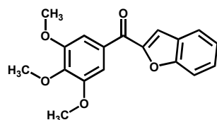
CTR 103
