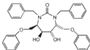
Aha001 (1AJX)
