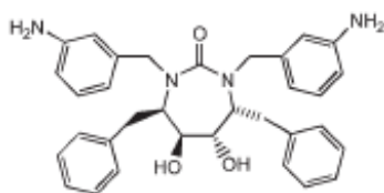
DMP450 (1DMP)
