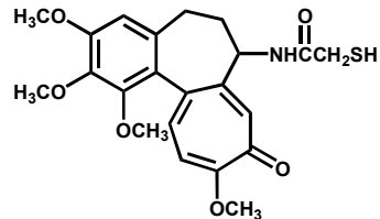
CTR 106
