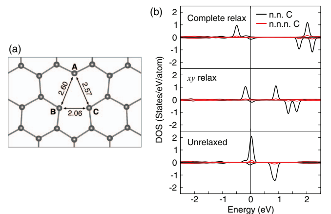
FIG. 2. (a) The local relaxation of graphene sheet with a monovacancy obtained from our calculations, where the grey balls represent the carbon atoms. The relative bond lengths of carbon atoms in close proximity to the vacancy and marked as A, B, and C are shown in Table II. (b) The density of states (DOS) for the unrelaxed (lower panel), relaxation constrained to xy -plane (middle panel), and free relaxation (upper panel) of graphene sheet having monovacancy is shown, respectively. The dark solid line (black) indicates the average DOS for carbon atoms nearest neighbor to the vacancy (n.n. C), while the light solid line (red) shows the DOS for the C atoms occupying the next nearest neighbor positions from the vacancy (n.n.n. C). The vertical line represents the Fermi level which is fixed to zero.
