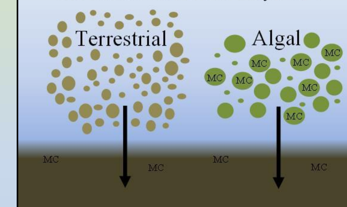
Sources of OM in the Sediments of the James River Estuary, VA
